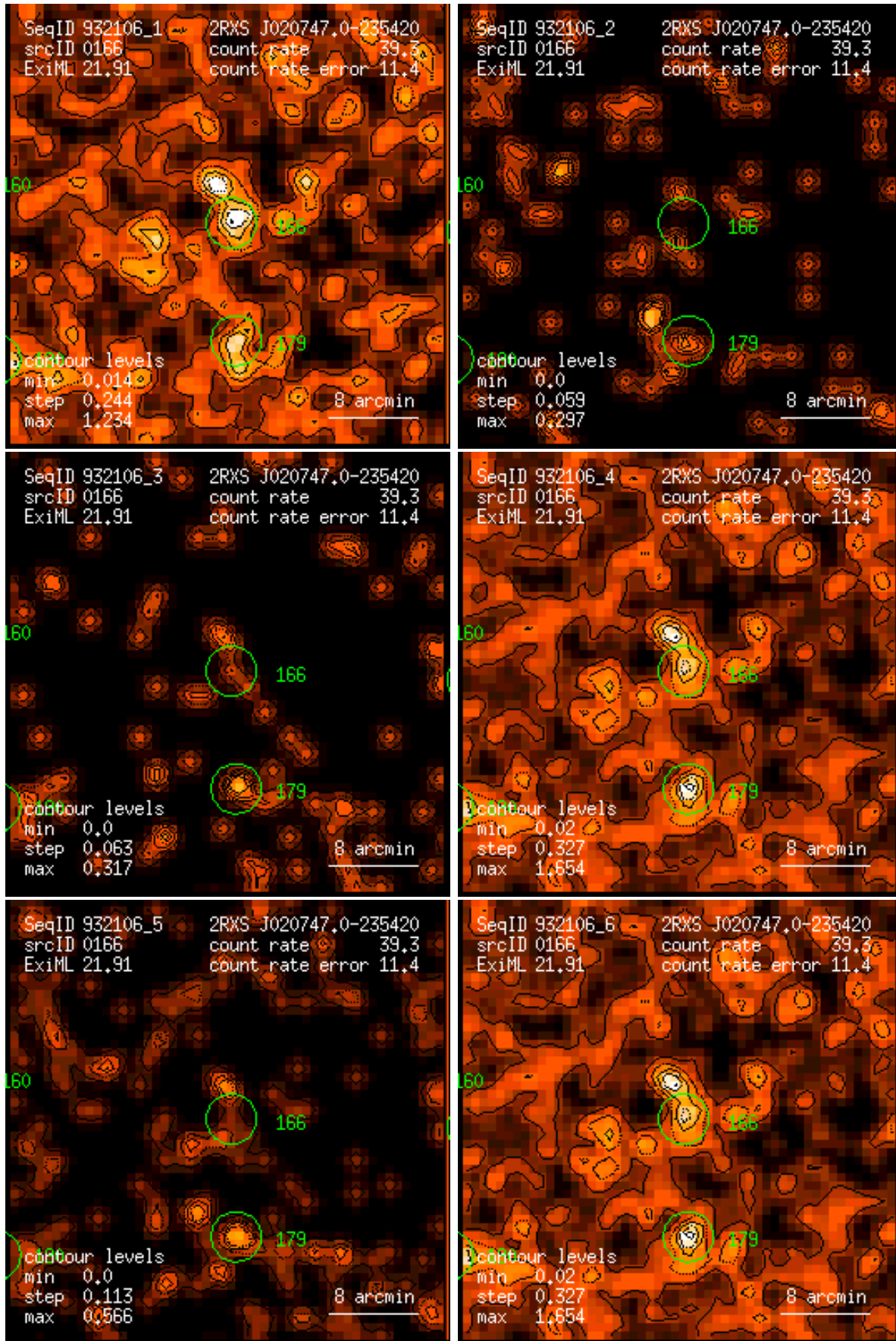
Figure 166: RASS 932106: detection 0166: band rate images, Gaussian filter: (1) PSPC channels 11 – 41, (2) 52 – 90, (3) 91 – 201, (4) 11 – 235, (5) 52 – 201, (6) 11 – 201. Broad band rates in counts/ks. Band rate contour levels in counts/ks/arcmin 2 .
