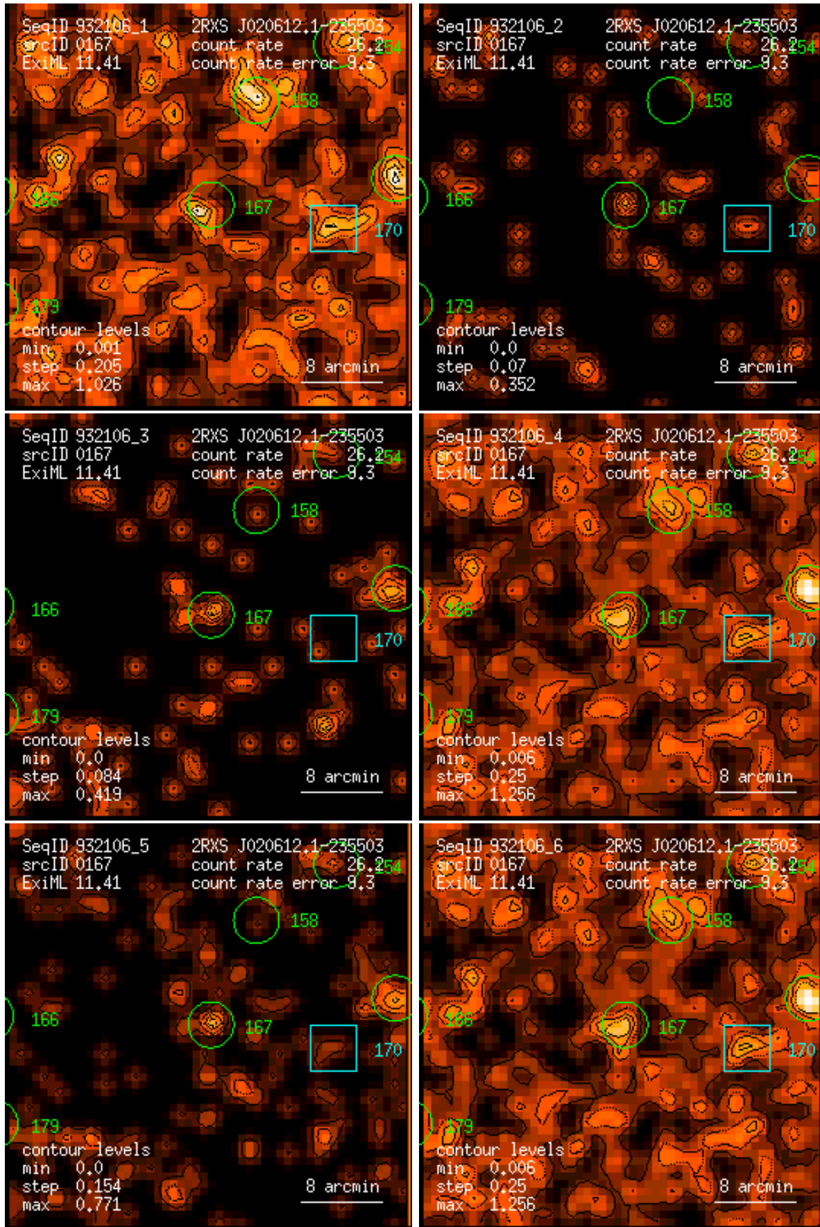
Figure 167: RASS 932106: detection 0167: band rate images, Gaussian filter: (1) PSPC channels 11 – 41, (2) 52 – 90, (3) 91 – 201, (4) 11 – 235, (5) 52 – 201, (6) 11 – 201. Broad band rates in counts/ks. Band rate contour levels in counts/ks/arcmin 2 .
