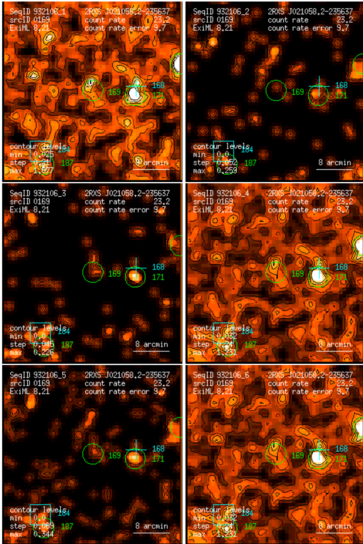
Figure 169: RASS 932106: detection 0169: band rate images, Gaussian filter: (1) PSPC channels 11 – 41, (2) 52 – 90, (3) 91 – 201, (4) 11 – 235, (5) 52 – 201, (6) 11 – 201. Broad band rates in counts/ks. Band rate contour levels in counts/ks/arcmin 2 .
