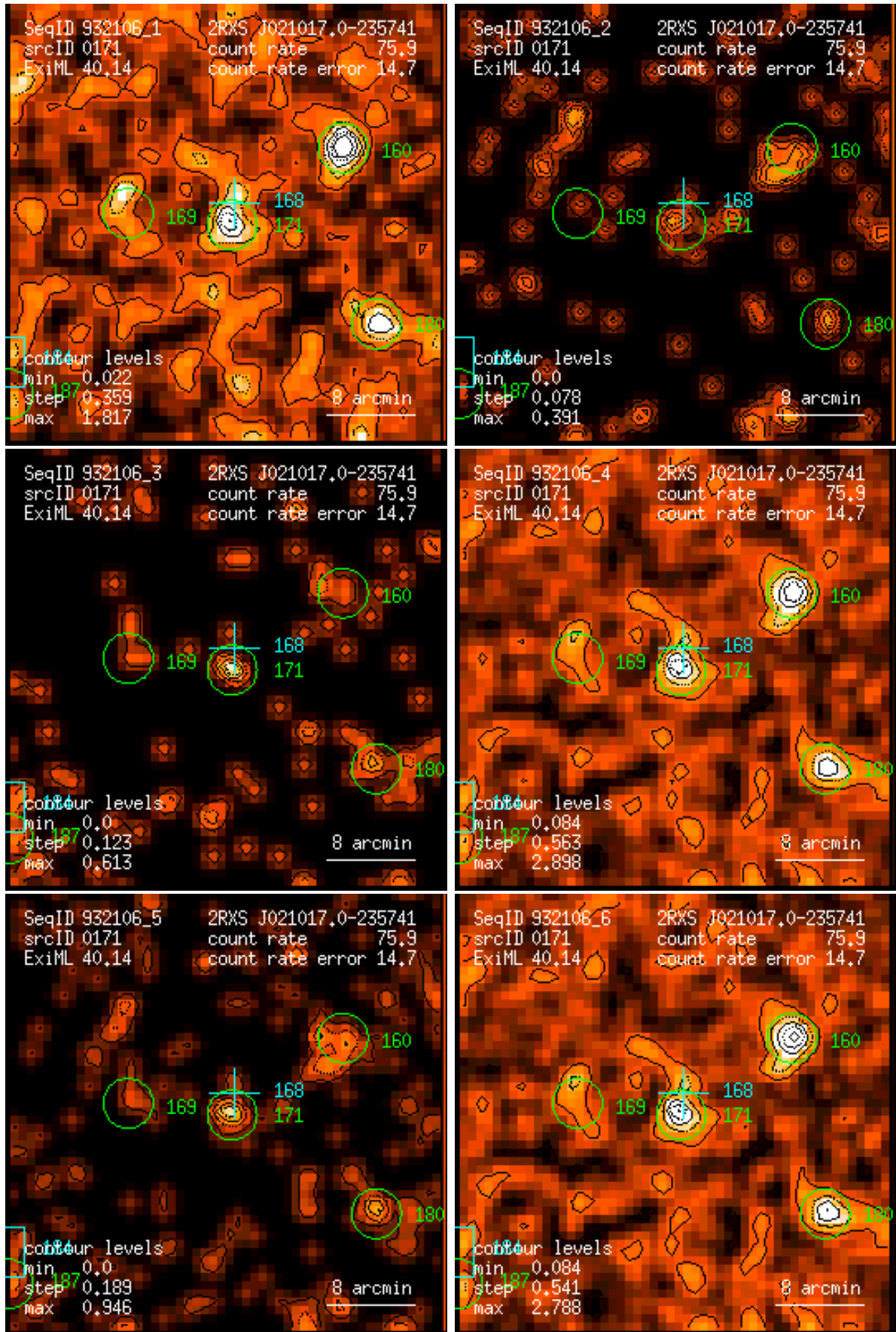
Figure 171: RASS 932106: detection 0171: band rate images, Gaussian filter: (1) PSPC channels 11 – 41, (2) 52 – 90, (3) 91 – 201, (4) 11 – 235, (5) 52 – 201, (6) 11 – 201. Broad band rates in counts/ks. Band rate contour levels in counts/ks/arcmin 2 .
