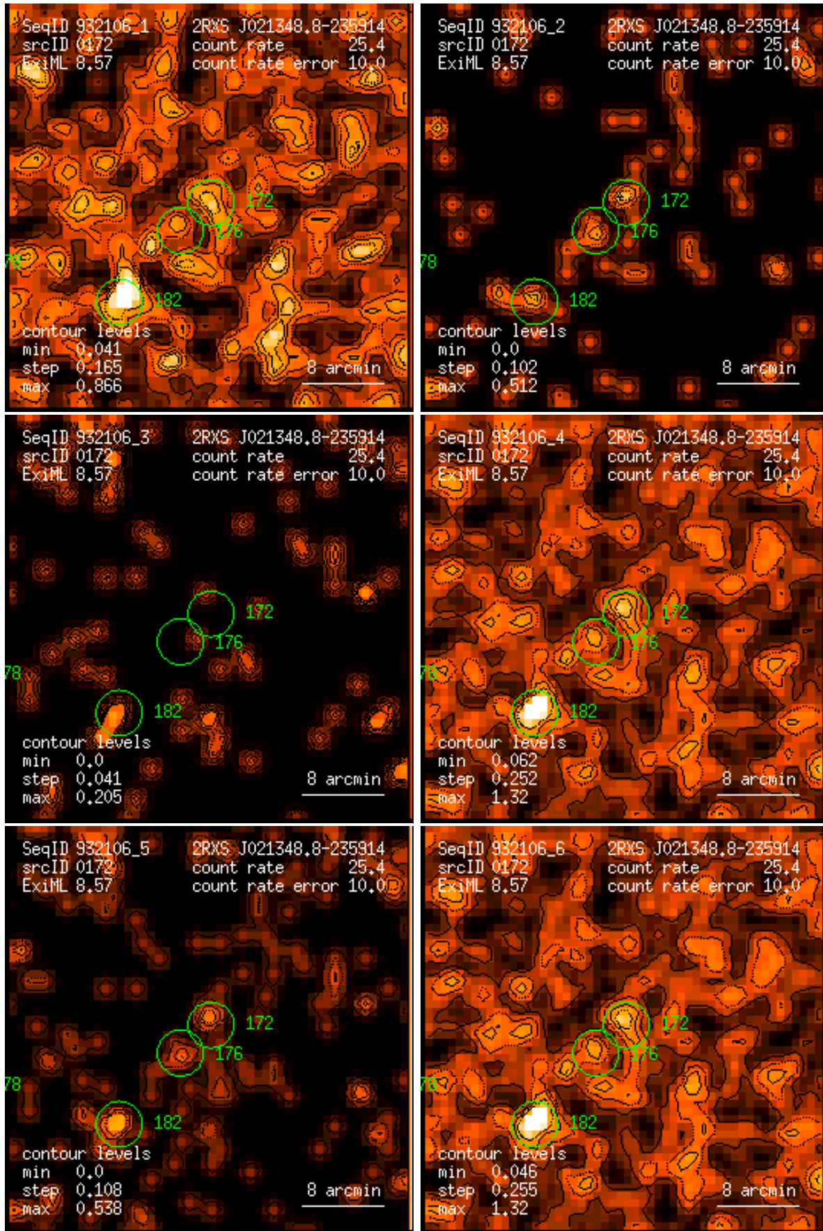
Figure 172: RASS 932106: detection 0172: band rate images, Gaussian filter: (1) PSPC channels 11 – 41, (2) 52 – 90, (3) 91 – 201, (4) 11 – 235, (5) 52 – 201, (6) 11 – 201. Broad band rates in counts/ks. Band rate contour levels in counts/ks/arcmin 2 .
