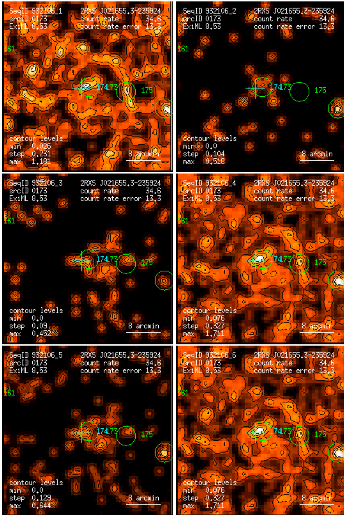
Figure 173: RASS 932106: detection 0173: band rate images, Gaussian filter: (1) PSPC channels 11 – 41, (2) 52 – 90, (3) 91 – 201, (4) 11 – 235, (5) 52 – 201, (6) 11 – 201. Broad band rates in counts/ks. Band rate contour levels in counts/ks/arcmin 2 .
