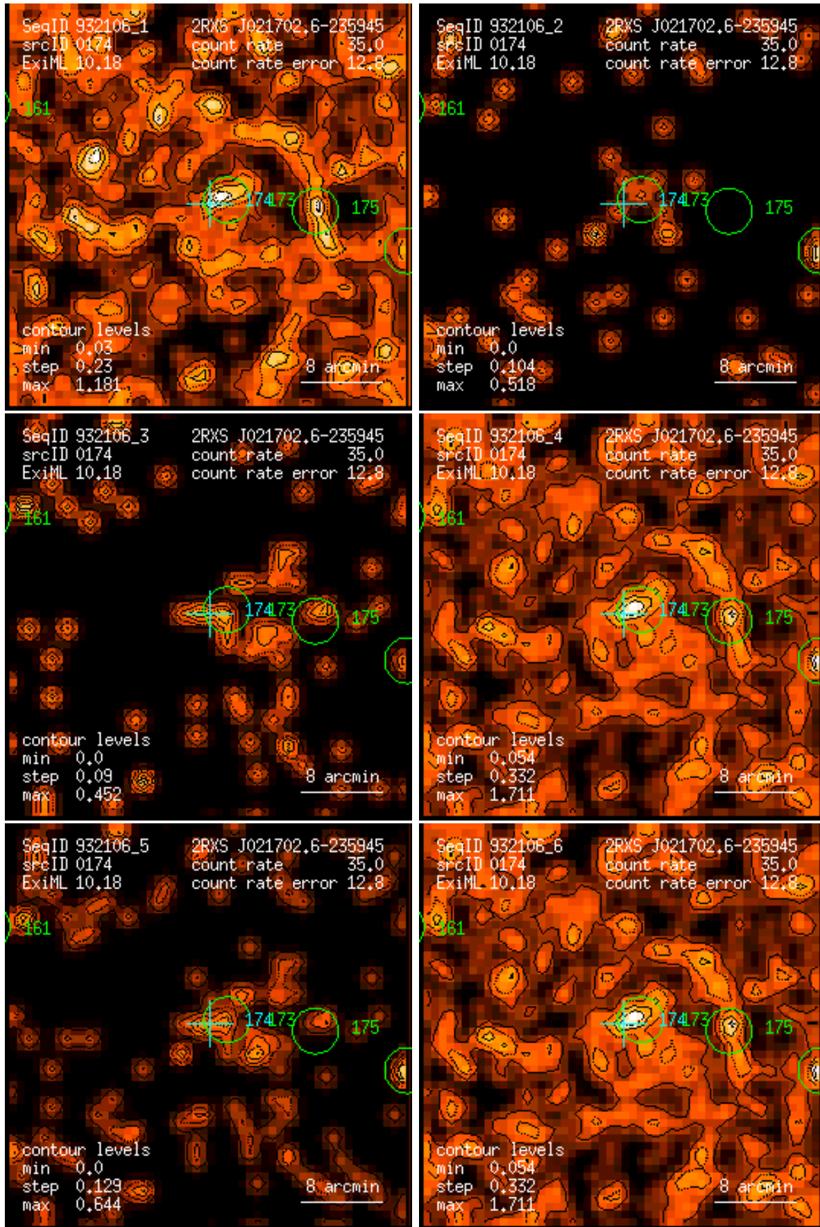
Figure 174: RASS 932106: detection 0174: band rate images, Gaussian filter: (1) PSPC channels 11 – 41, (2) 52 – 90, (3) 91 – 201, (4) 11 – 235, (5) 52 – 201, (6) 11 – 201. Broad band rates in counts/ks. Band rate contour levels in counts/ks/arcmin 2 .
