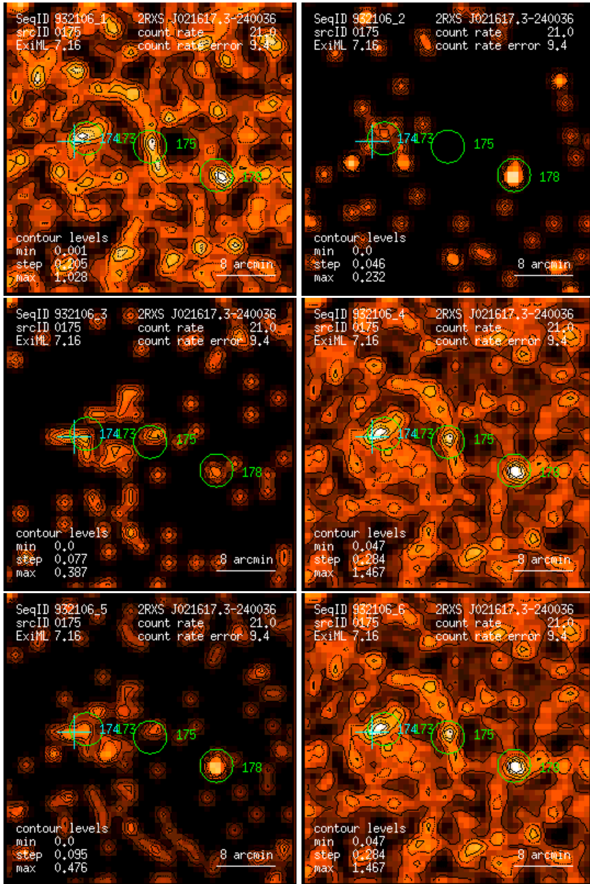
Figure 175: RASS 932106: detection 0175: band rate images, Gaussian filter: (1) PSPC channels 11 – 41, (2) 52 – 90, (3) 91 – 201, (4) 11 – 235, (5) 52 – 201, (6) 11 – 201. Broad band rates in counts/ks. Band rate contour levels in counts/ks/arcmin 2 .
