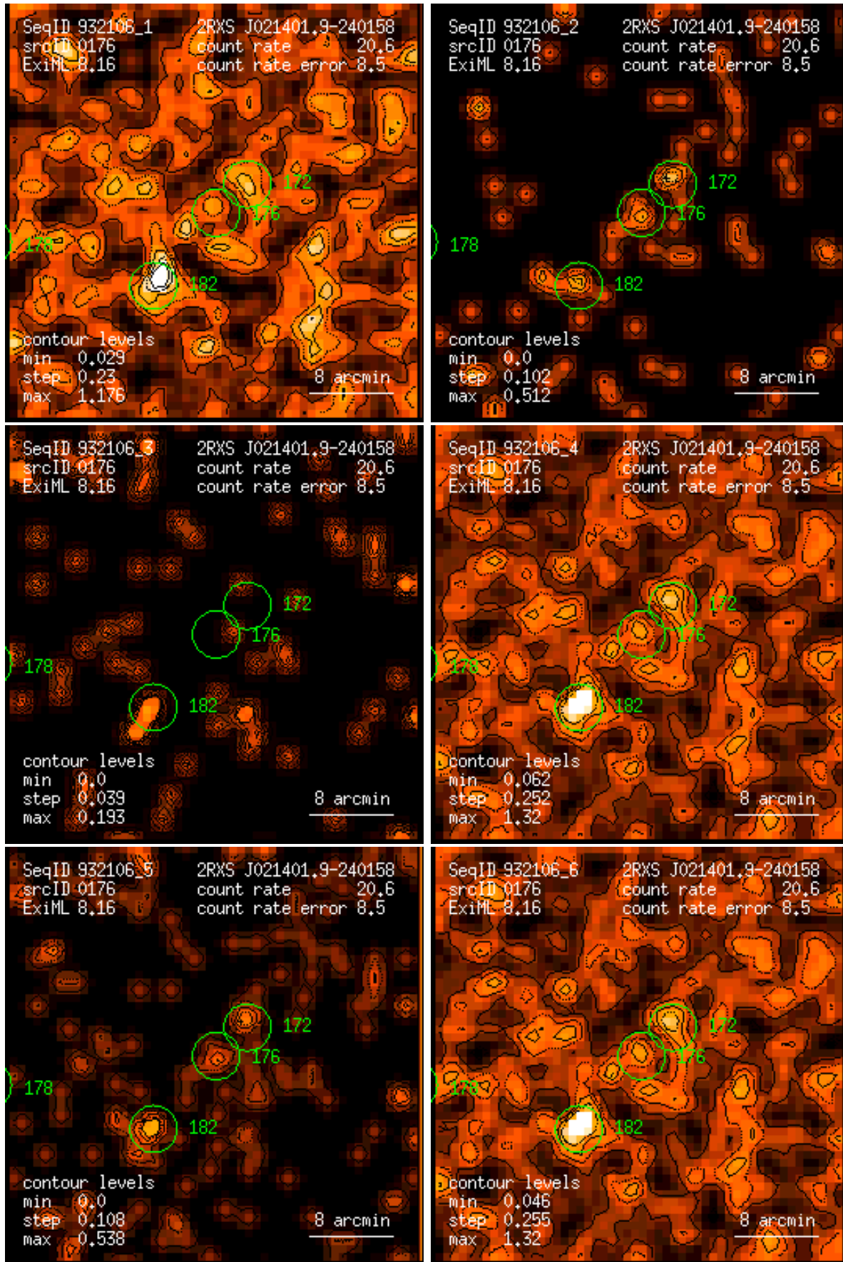
Figure 176: RASS 932106: detection 0176: band rate images, Gaussian filter: (1) PSPC channels 11 – 41, (2) 52 – 90, (3) 91 – 201, (4) 11 – 235, (5) 52 – 201, (6) 11 – 201. Broad band rates in counts/ks. Band rate contour levels in counts/ks/arcmin 2 .
