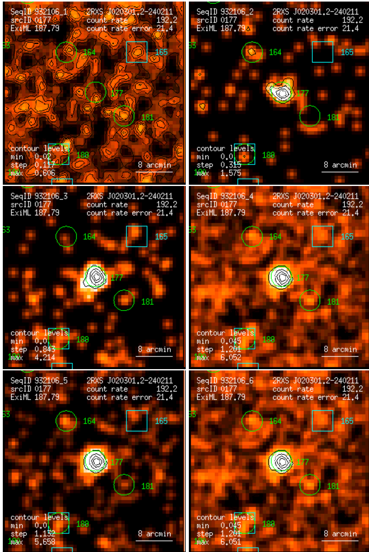
Figure 177: RASS 932106: detection 0177: band rate images, Gaussian filter: (1) PSPC channels 11 – 41, (2) 52 – 90, (3) 91 – 201, (4) 11 – 235, (5) 52 – 201, (6) 11 – 201. Broad band rates in counts/ks. Band rate contour levels in counts/ks/arcmin 2 .
