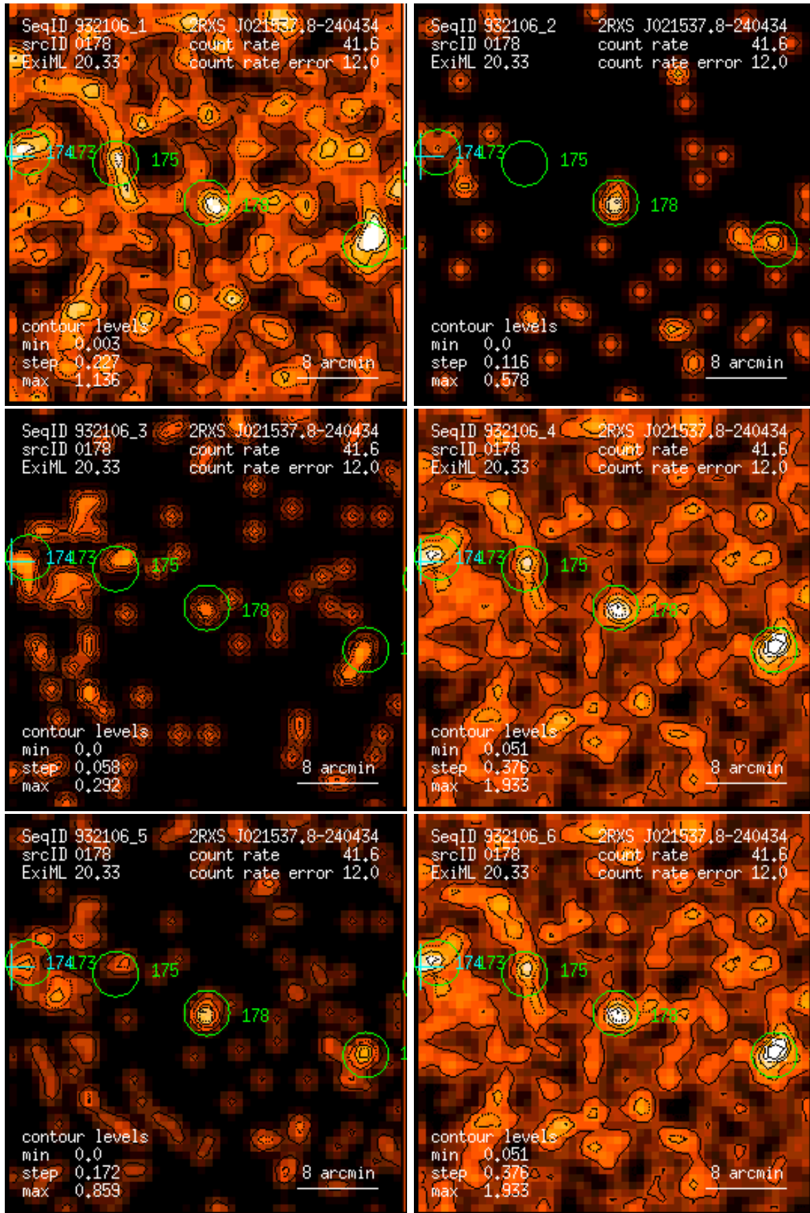
Figure 178: RASS 932106: detection 0178: band rate images, Gaussian filter: (1) PSPC channels 11 – 41, (2) 52 – 90, (3) 91 – 201, (4) 11 – 235, (5) 52 – 201, (6) 11 – 201. Broad band rates in counts/ks. Band rate contour levels in counts/ks/arcmin 2 .
