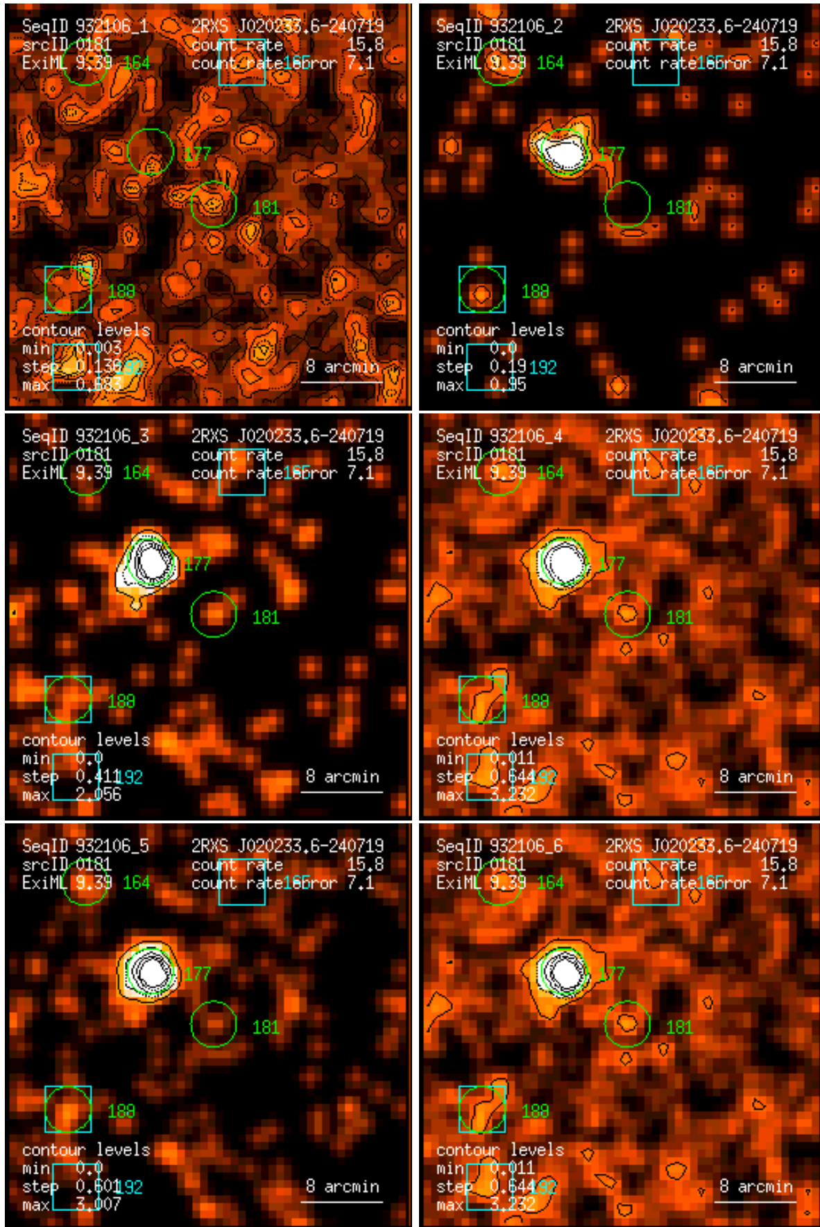
Figure 181: RASS 932106: detection 0181: band rate images, Gaussian filter: (1) PSPC channels 11 – 41, (2) 52 – 90, (3) 91 – 201, (4) 11 – 235, (5) 52 – 201, (6) 11 – 201. Broad band rates in counts/ks. Band rate contour levels in counts/ks/arcmin 2 .
