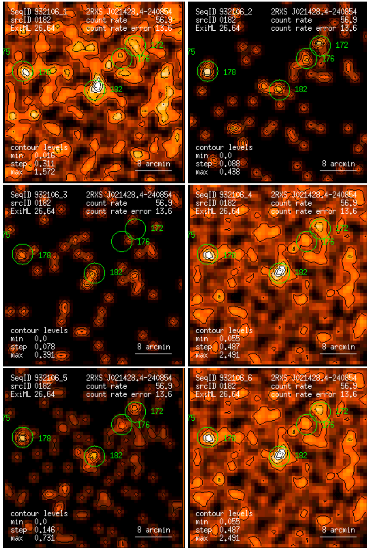
Figure 182: RASS 932106: detection 0182: band rate images, Gaussian filter: (1) PSPC channels 11 – 41, (2) 52 – 90, (3) 91 – 201, (4) 11 – 235, (5) 52 – 201, (6) 11 – 201. Broad band rates in counts/ks. Band rate contour levels in counts/ks/arcmin 2 .
