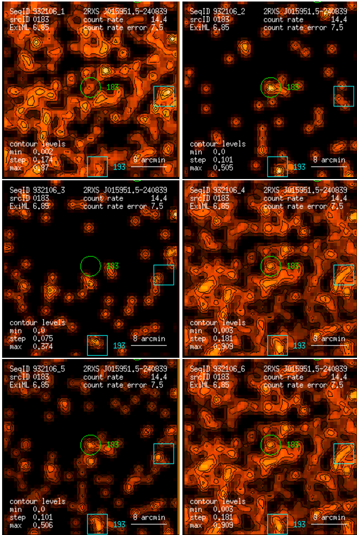
Figure 183: RASS 932106: detection 0183: band rate images, Gaussian filter: (1) PSPC channels 11 – 41, (2) 52 – 90, (3) 91 – 201, (4) 11 – 235, (5) 52 – 201, (6) 11 – 201. Broad band rates in counts/ks. Band rate contour levels in counts/ks/arcmin 2 .
