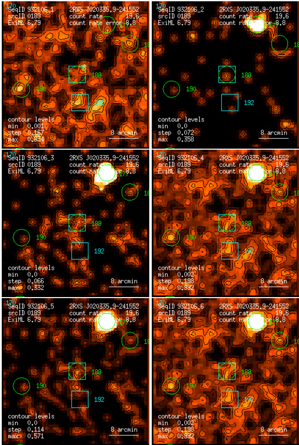
Figure 189: RASS 932106: detection 0189: band rate images, Gaussian filter: (1) PSPC channels 11 – 41, (2) 52 – 90, (3) 91 – 201, (4) 11 – 235, (5) 52 – 201, (6) 11 – 201. Broad band rates in counts/ks. Band rate contour levels in counts/ks/arcmin 2 .
