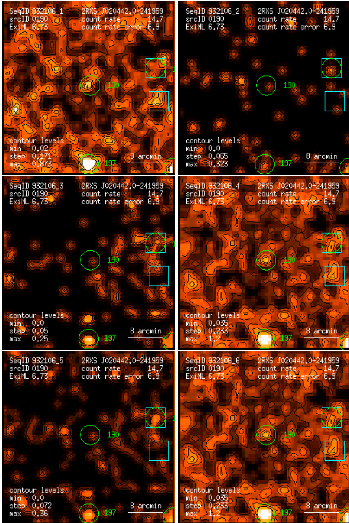
Figure 190: RASS 932106: detection 0190: band rate images, Gaussian filter: (1) PSPC channels 11 – 41, (2) 52 – 90, (3) 91 – 201, (4) 11 – 235, (5) 52 – 201, (6) 11 – 201. Broad band rates in counts/ks. Band rate contour levels in counts/ks/arcmin 2 .
