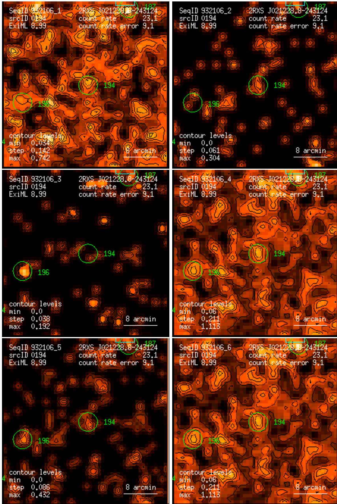
Figure 194: RASS 932106: detection 0194: band rate images, Gaussian filter: (1) PSPC channels 11 – 41, (2) 52 – 90, (3) 91 – 201, (4) 11 – 235, (5) 52 – 201, (6) 11 – 201. Broad band rates in counts/ks. Band rate contour levels in counts/ks/arcmin 2 .
