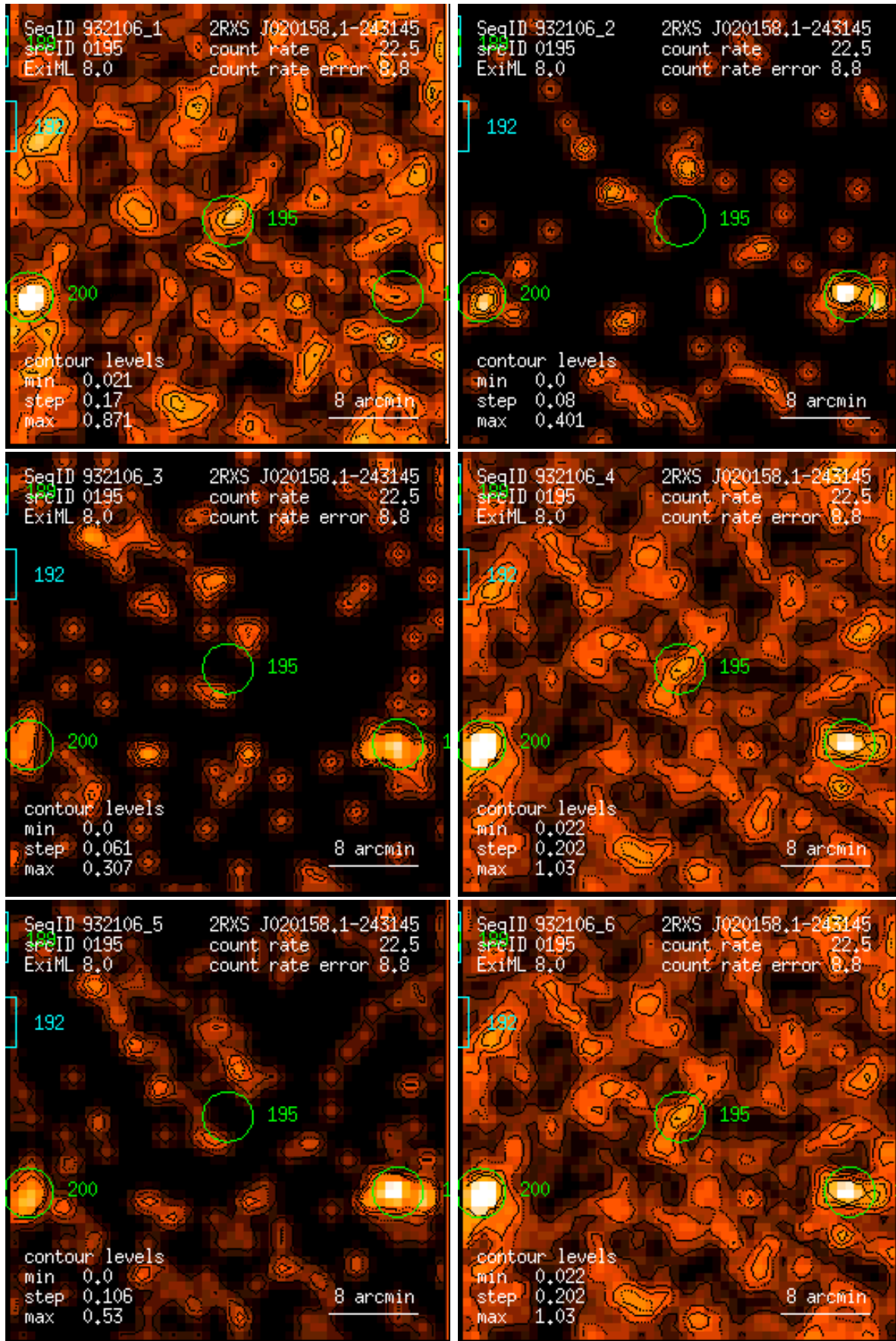
Figure 195: RASS 932106: detection 0195: band rate images, Gaussian filter: (1) PSPC channels 11 – 41, (2) 52 – 90, (3) 91 – 201, (4) 11 – 235, (5) 52 – 201, (6) 11 – 201. Broad band rates in counts/ks. Band rate contour levels in counts/ks/arcmin 2 .
