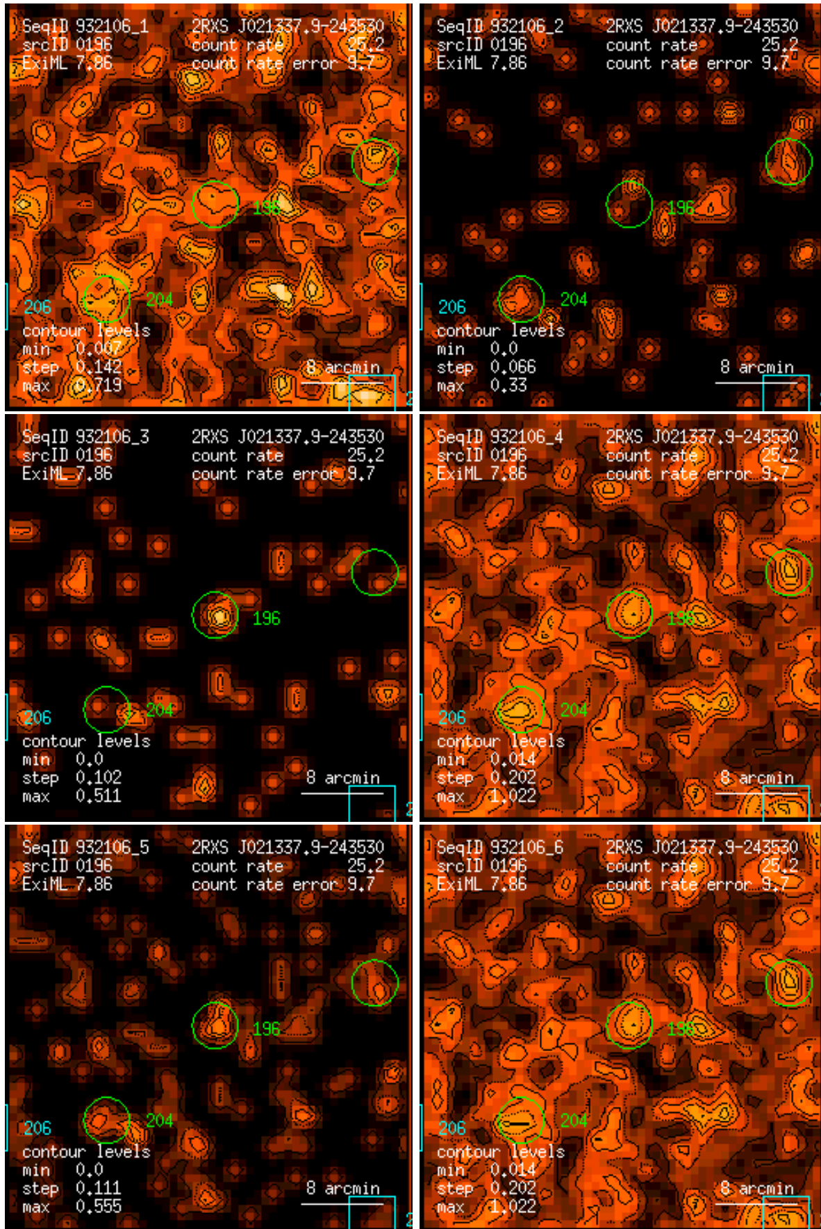
Figure 196: RASS 932106: detection 0196: band rate images, Gaussian filter: (1) PSPC channels 11 – 41, (2) 52 – 90, (3) 91 – 201, (4) 11 – 235, (5) 52 – 201, (6) 11 – 201. Broad band rates in counts/ks. Band rate contour levels in counts/ks/arcmin 2 .
