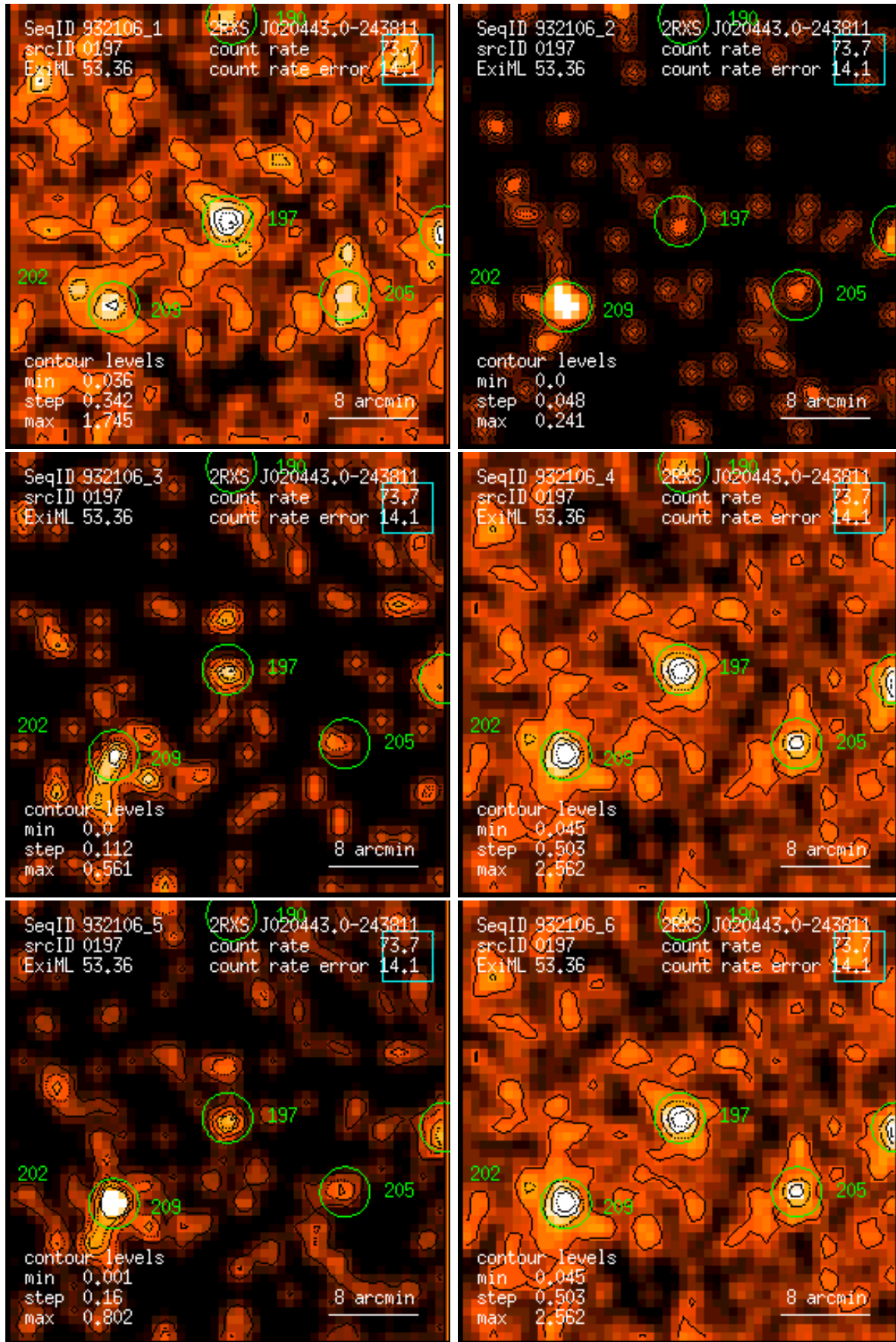
Figure 197: RASS 932106: detection 0197: band rate images, Gaussian filter: (1) PSPC channels 11 – 41, (2) 52 – 90, (3) 91 – 201, (4) 11 – 235, (5) 52 – 201, (6) 11 – 201. Broad band rates in counts/ks. Band rate contour levels in counts/ks/arcmin 2 .
