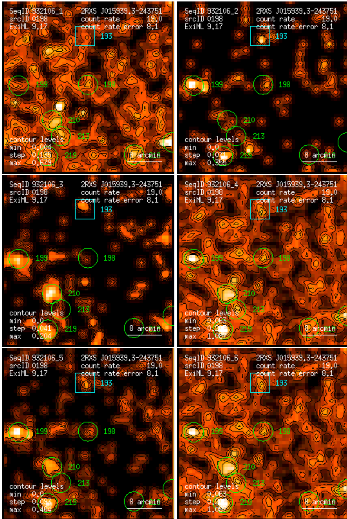
Figure 198: RASS 932106: detection 0198: band rate images, Gaussian filter: (1) PSPC channels 11 – 41, (2) 52 – 90, (3) 91 – 201, (4) 11 – 235, (5) 52 – 201, (6) 11 – 201. Broad band rates in counts/ks. Band rate contour levels in counts/ks/arcmin 2 .
