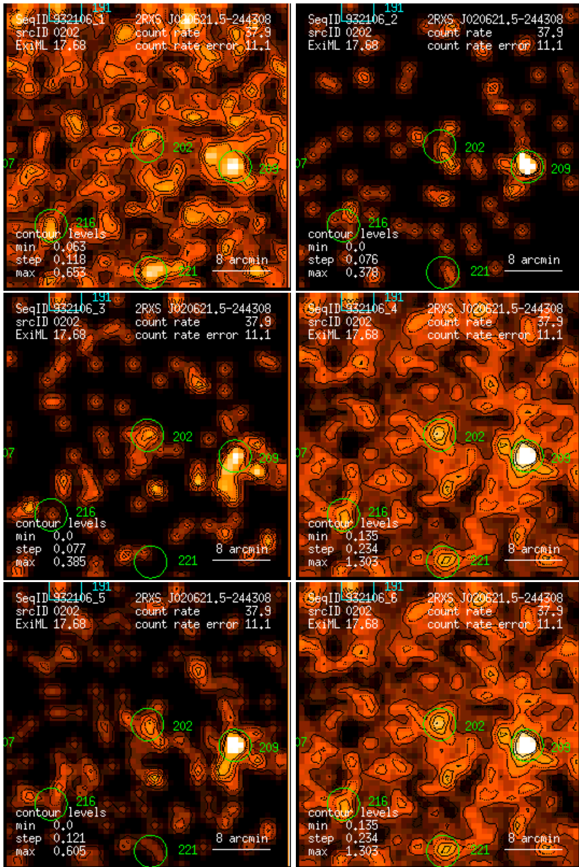
Figure 202: RASS 932106: detection 0202: band rate images, Gaussian filter: (1) PSPC channels 11 – 41, (2) 52 – 90, (3) 91 – 201, (4) 11 – 235, (5) 52 – 201, (6) 11 – 201. Broad band rates in counts/ks. Band rate contour levels in counts/ks/arcmin 2 .
