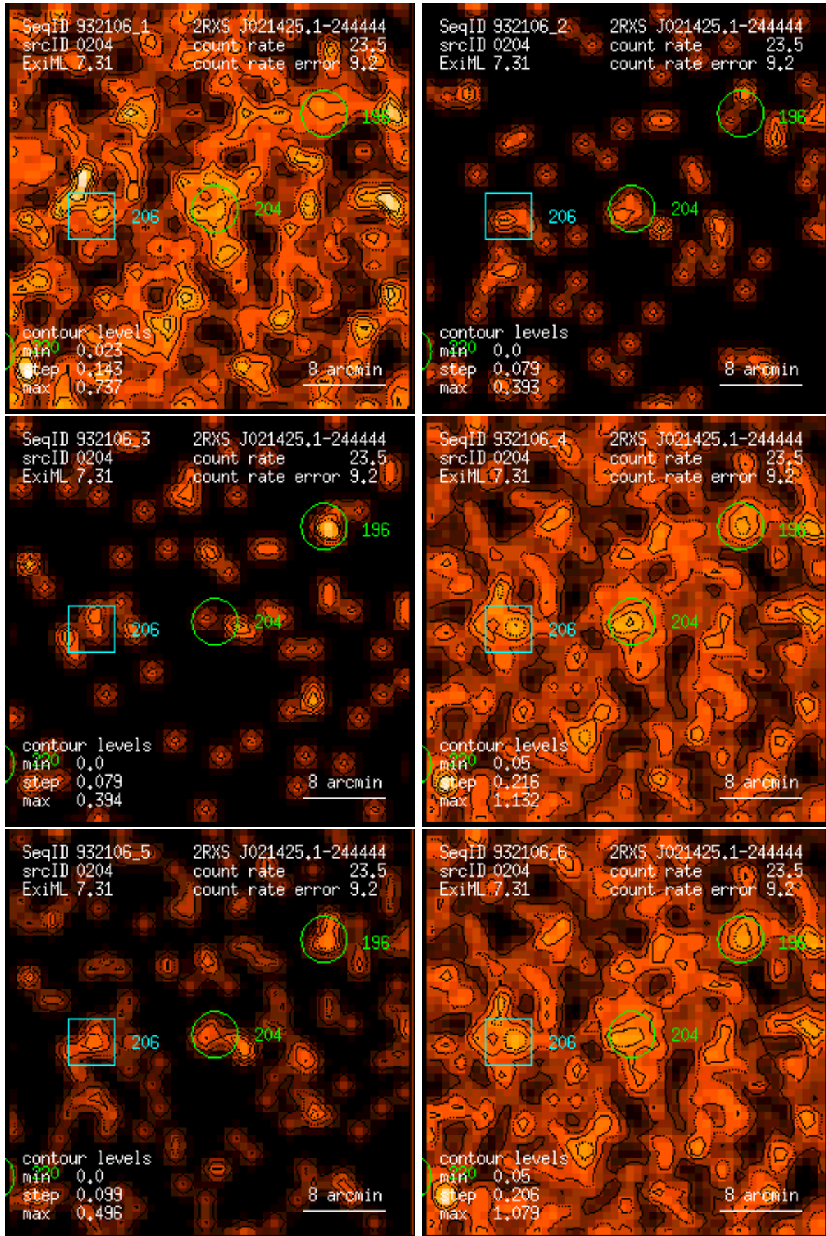
Figure 204: RASS 932106: detection 0204: band rate images, Gaussian filter: (1) PSPC channels 11 – 41, (2) 52 – 90, (3) 91 – 201, (4) 11 – 235, (5) 52 – 201, (6) 11 – 201. Broad band rates in counts/ks. Band rate contour levels in counts/ks/arcmin 2 .
