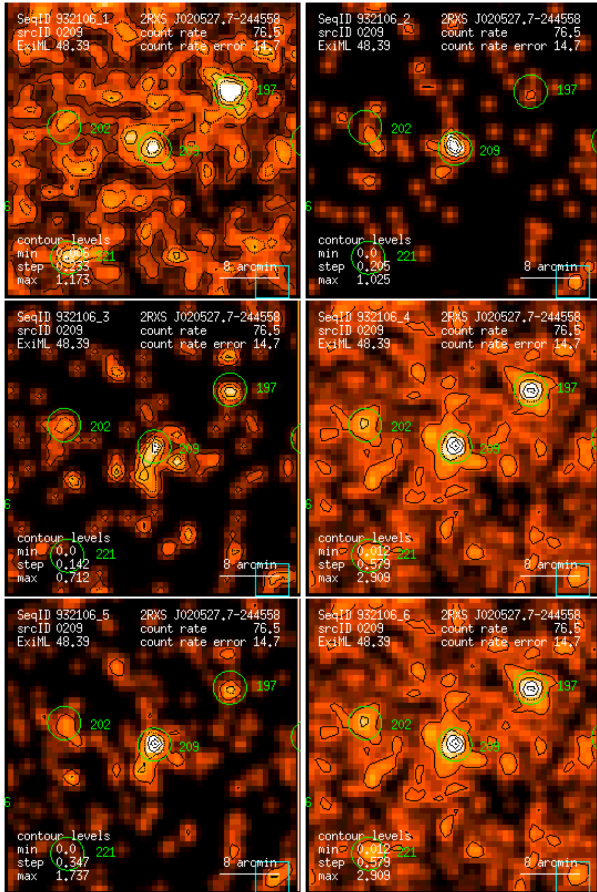
Figure 209: RASS 932106: detection 0209: band rate images, Gaussian filter: (1) PSPC channels 11 – 41, (2) 52 – 90, (3) 91 – 201, (4) 11 – 235, (5) 52 – 201, (6) 11 – 201. Broad band rates in counts/ks. Band rate contour levels in counts/ks/arcmin 2 .
