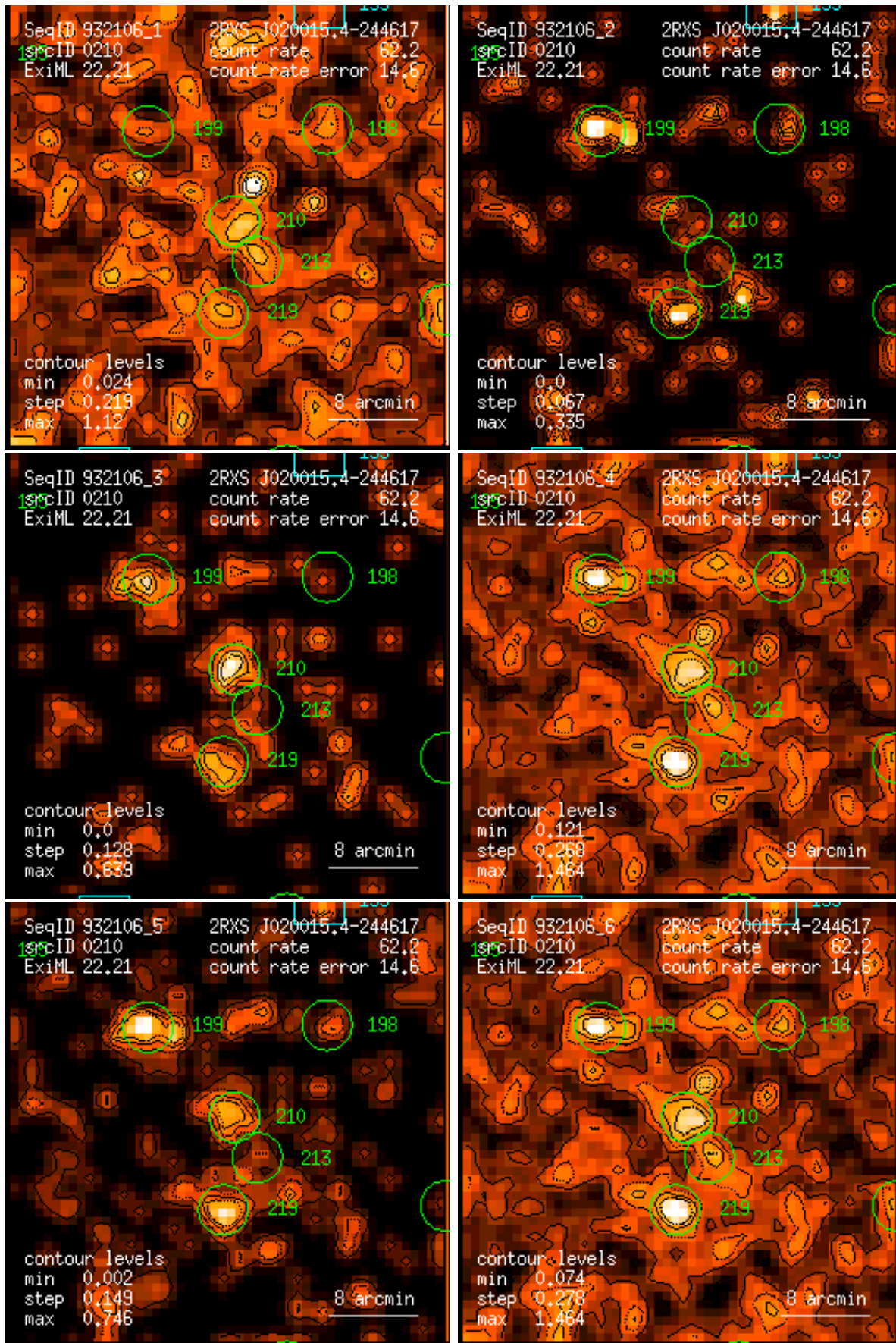
Figure 210: RASS 932106: detection 0210: band rate images, Gaussian filter: (1) PSPC channels 11 – 41, (2) 52 – 90, (3) 91 – 201, (4) 11 – 235, (5) 52 – 201, (6) 11 – 201. Broad band rates in counts/ks. Band rate contour levels in counts/ks/arcmin 2 .
