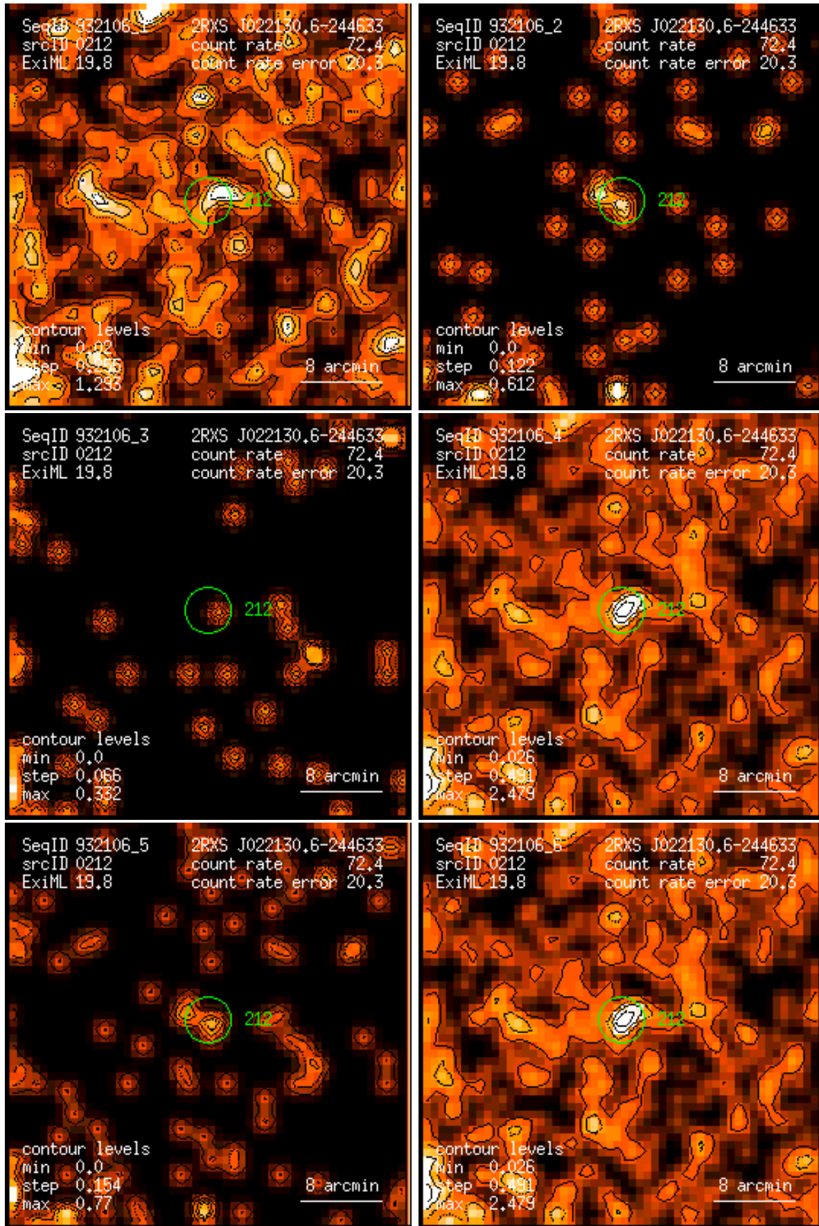
Figure 212: RASS 932106: detection 0212: band rate images, Gaussian filter: (1) PSPC channels 11 – 41, (2) 52 – 90, (3) 91 – 201, (4) 11 – 235, (5) 52 – 201, (6) 11 – 201. Broad band rates in counts/ks. Band rate contour levels in counts/ks/arcmin 2 .
