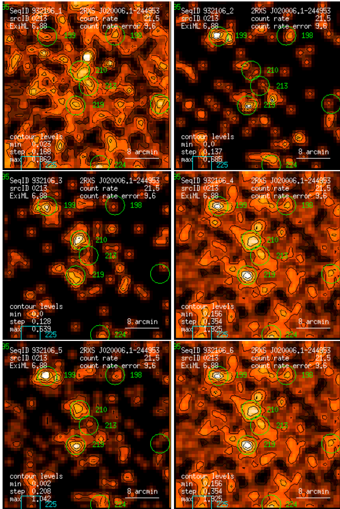
Figure 213: RASS 932106: detection 0213: band rate images, Gaussian filter: (1) PSPC channels 11 – 41, (2) 52 – 90, (3) 91 – 201, (4) 11 – 235, (5) 52 – 201, (6) 11 – 201. Broad band rates in counts/ks. Band rate contour levels in counts/ks/arcmin 2 .
