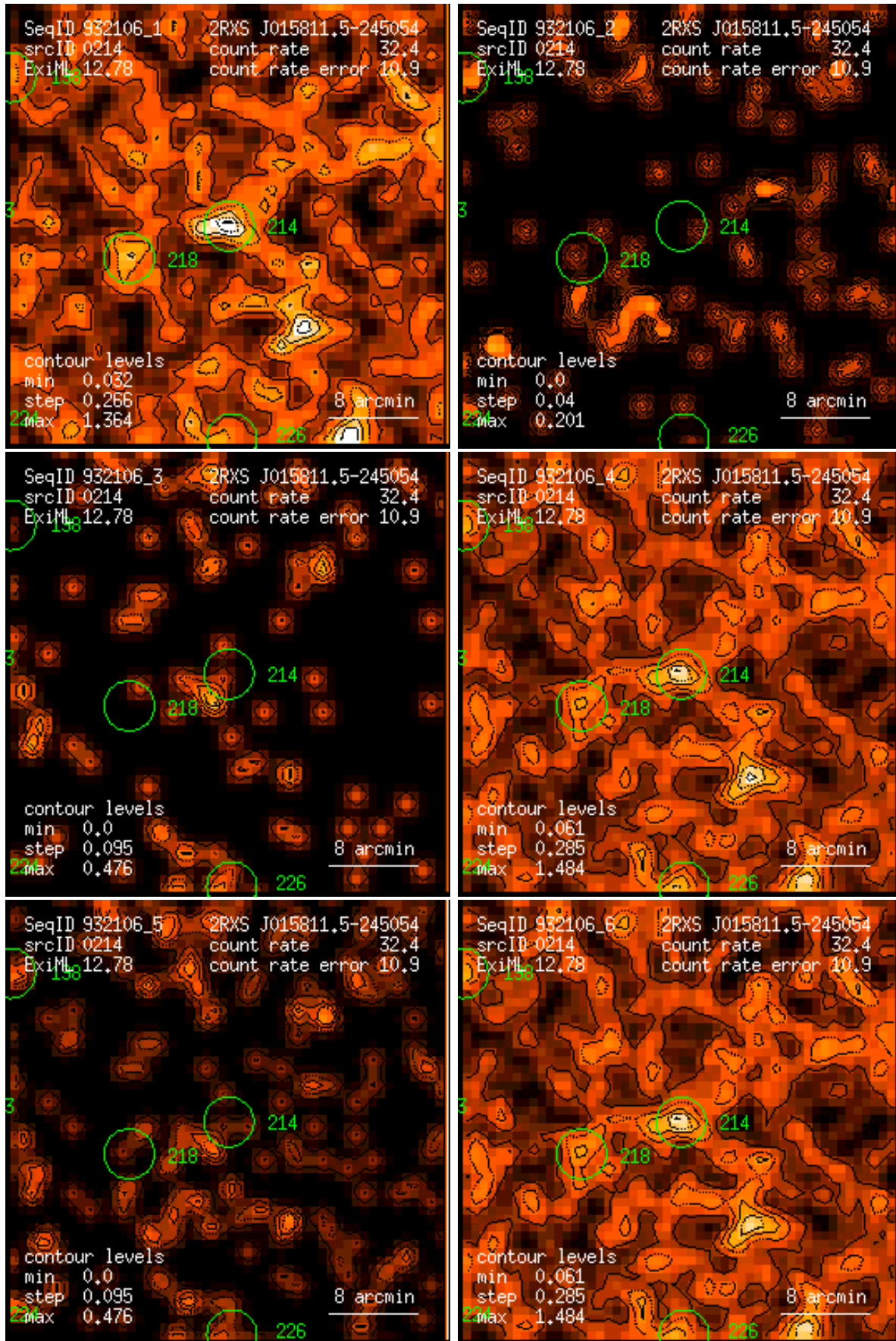
Figure 214: RASS 932106: detection 0214: band rate images, Gaussian filter: (1) PSPC channels 11 – 41, (2) 52 – 90, (3) 91 – 201, (4) 11 – 235, (5) 52 – 201, (6) 11 – 201. Broad band rates in counts/ks. Band rate contour levels in counts/ks/arcmin 2 .
