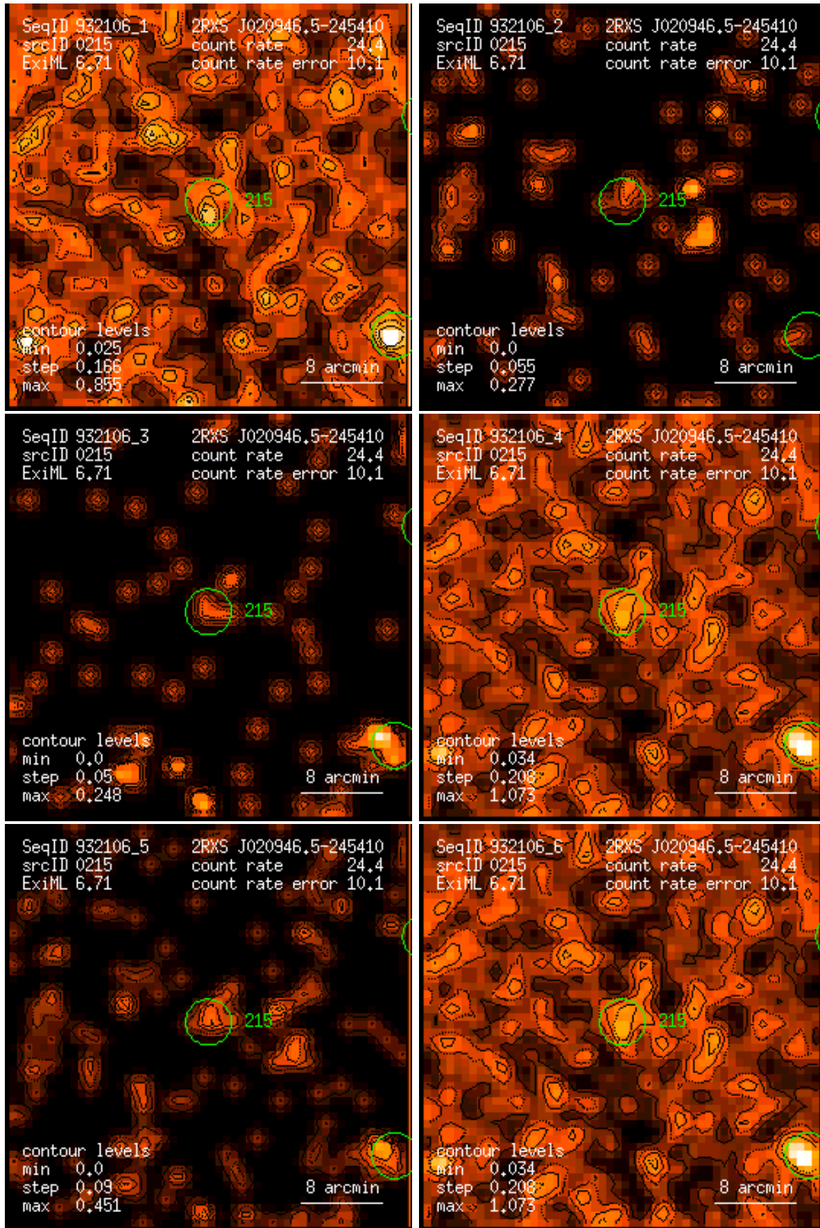
Figure 215: RASS 932106: detection 0215: band rate images, Gaussian filter: (1) PSPC channels 11 – 41, (2) 52 – 90, (3) 91 – 201, (4) 11 – 235, (5) 52 – 201, (6) 11 – 201. Broad band rates in counts/ks. Band rate contour levels in counts/ks/arcmin 2 .
