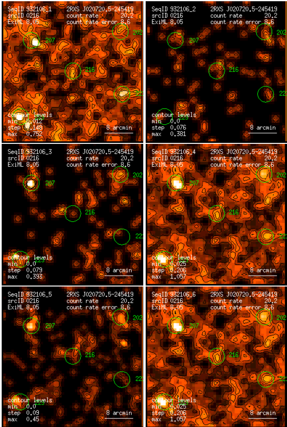
Figure 216: RASS 932106: detection 0216: band rate images, Gaussian filter: (1) PSPC channels 11 – 41, (2) 52 – 90, (3) 91 – 201, (4) 11 – 235, (5) 52 – 201, (6) 11 – 201. Broad band rates in counts/ks. Band rate contour levels in counts/ks/arcmin 2 .
