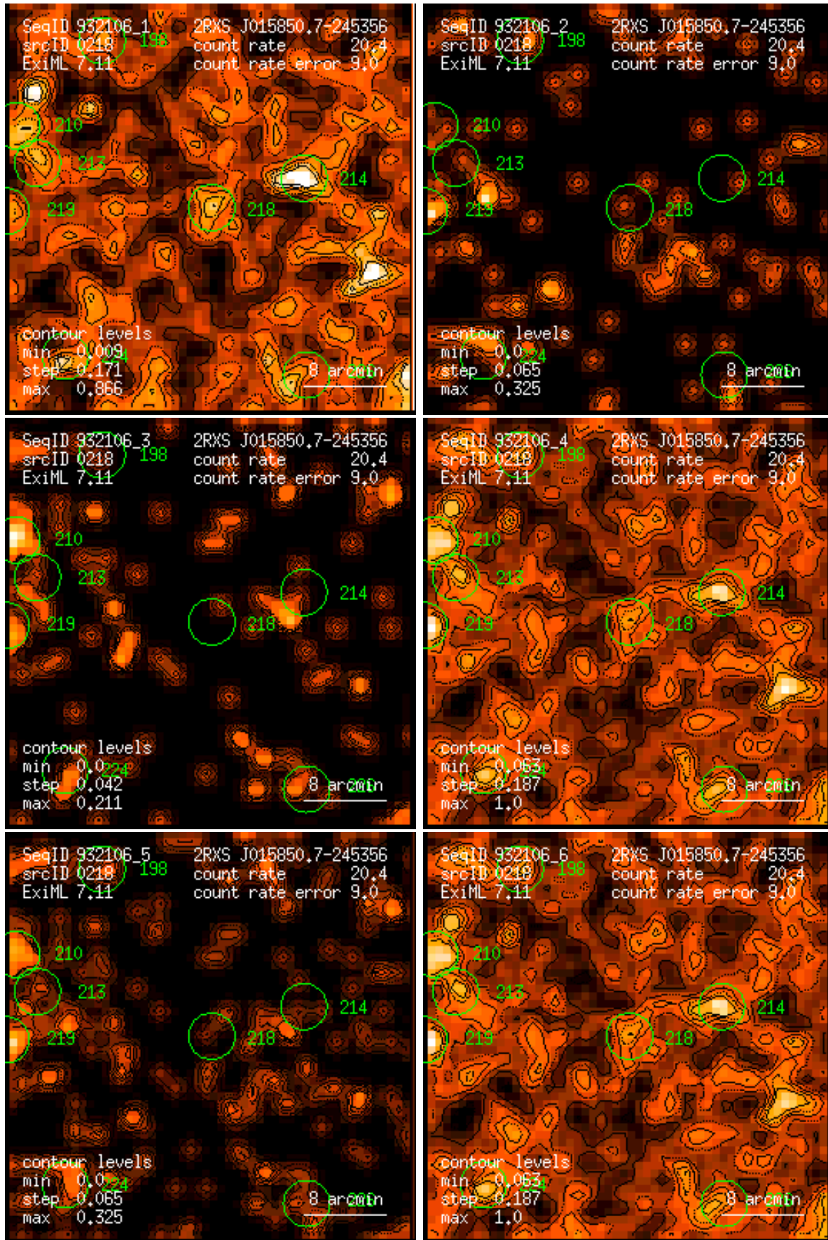
Figure 218: RASS 932106: detection 0218: band rate images, Gaussian filter: (1) PSPC channels 11 – 41, (2) 52 – 90, (3) 91 – 201, (4) 11 – 235, (5) 52 – 201, (6) 11 – 201. Broad band rates in counts/ks. Band rate contour levels in counts/ks/arcmin 2 .
