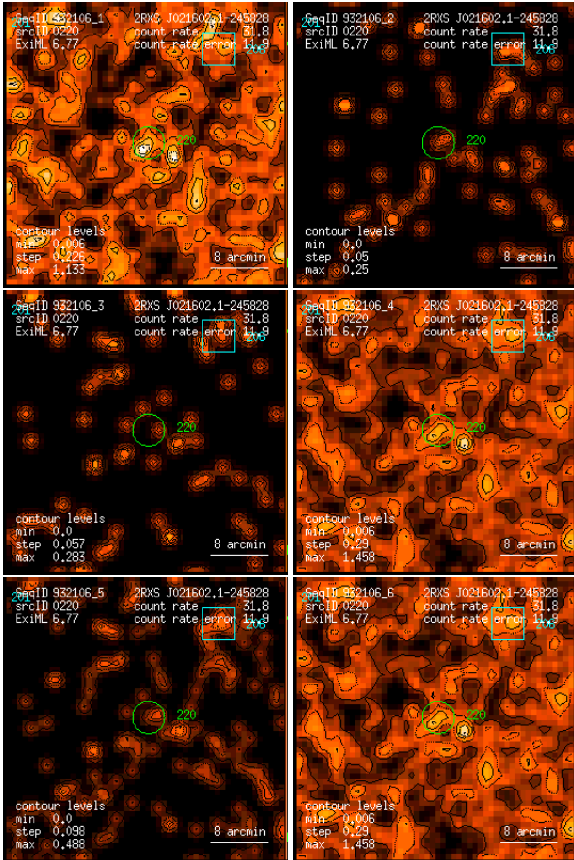
Figure 220: RASS 932106: detection 0220: band rate images, Gaussian filter: (1) PSPC channels 11 – 41, (2) 52 – 90, (3) 91 – 201, (4) 11 – 235, (5) 52 – 201, (6) 11 – 201. Broad band rates in counts/ks. Band rate contour levels in counts/ks/arcmin 2 .
