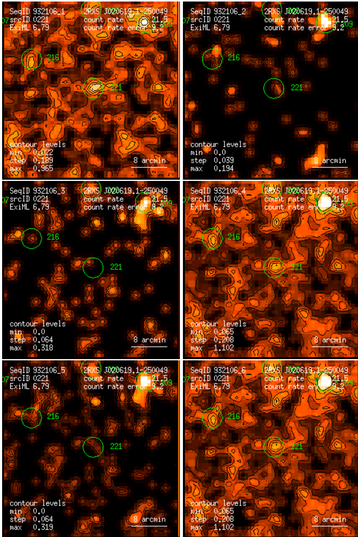
Figure 221: RASS 932106: detection 0221: band rate images, Gaussian filter: (1) PSPC channels 11 – 41, (2) 52 – 90, (3) 91 – 201, (4) 11 – 235, (5) 52 – 201, (6) 11 – 201. Broad band rates in counts/ks. Band rate contour levels in counts/ks/arcmin 2 .
