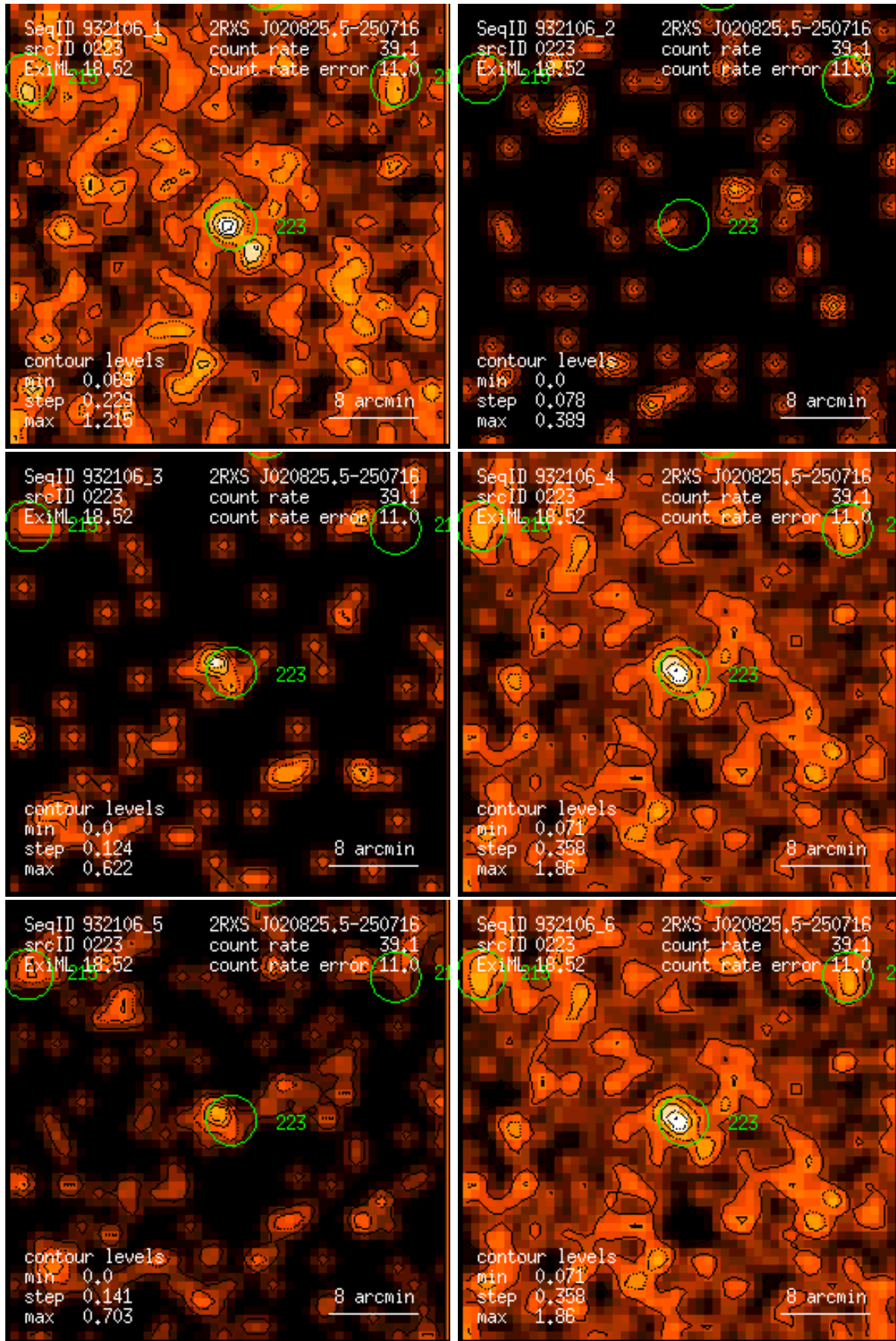
Figure 223: RASS 932106: detection 0223: band rate images, Gaussian filter: (1) PSPC channels 11 – 41, (2) 52 – 90, (3) 91 – 201, (4) 11 – 235, (5) 52 – 201, (6) 11 – 201. Broad band rates in counts/ks. Band rate contour levels in counts/ks/arcmin 2 .
