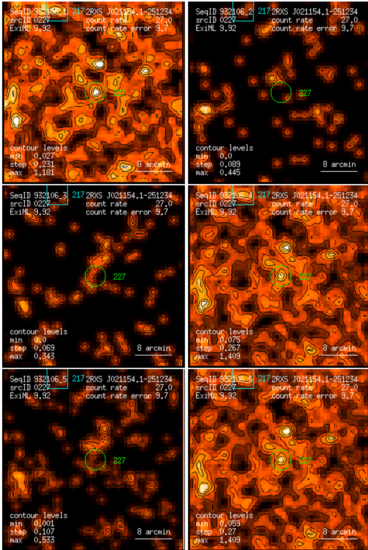
Figure 227: RASS 932106: detection 0227: band rate images, Gaussian filter: (1) PSPC channels 11 – 41, (2) 52 – 90, (3) 91 – 201, (4) 11 – 235, (5) 52 – 201, (6) 11 – 201. Broad band rates in counts/ks. Band rate contour levels in counts/ks/arcmin 2 .
