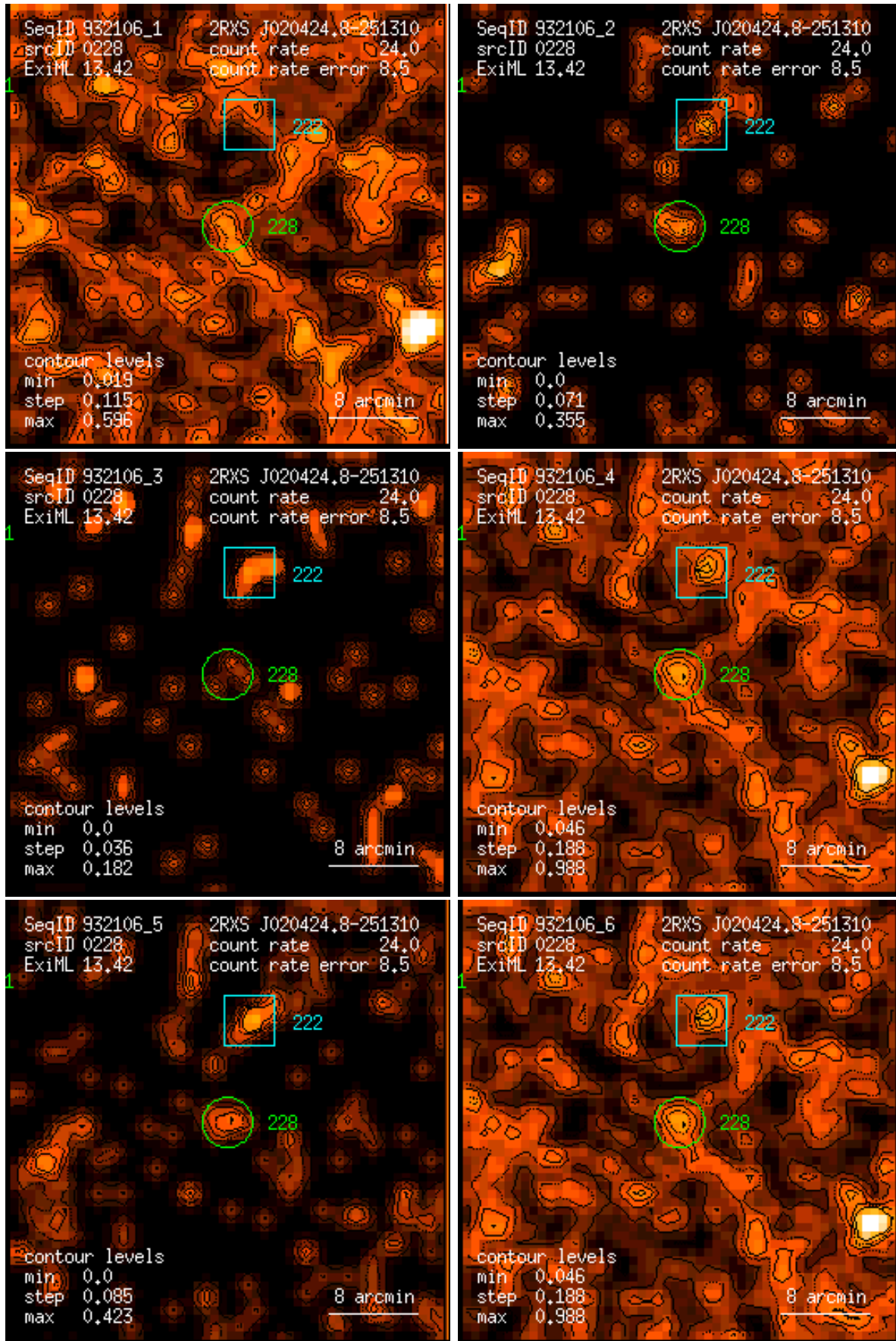
Figure 228: RASS 932106: detection 0228: band rate images, Gaussian filter: (1) PSPC channels 11 – 41, (2) 52 – 90, (3) 91 – 201, (4) 11 – 235, (5) 52 – 201, (6) 11 – 201. Broad band rates in counts/ks. Band rate contour levels in counts/ks/arcmin 2 .
