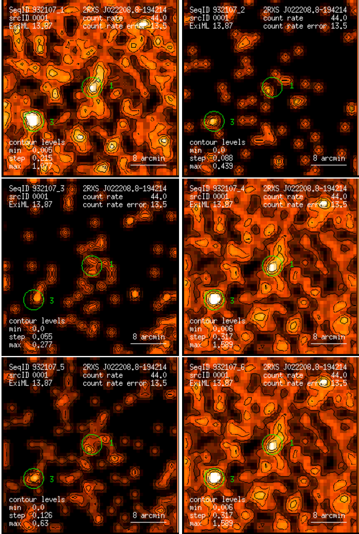
Figure 1: RASS 932107: detection 0001: band rate images, Gaussian filter: (1) PSPC channels 11 – 41, (2) 52 – 90, (3) 91 – 201, (4) 11 – 235, (5) 52 – 201, (6) 11 – 201. Broad band rates in counts/ks. Band rate contour levels in counts/ks/arcmin 2 .
