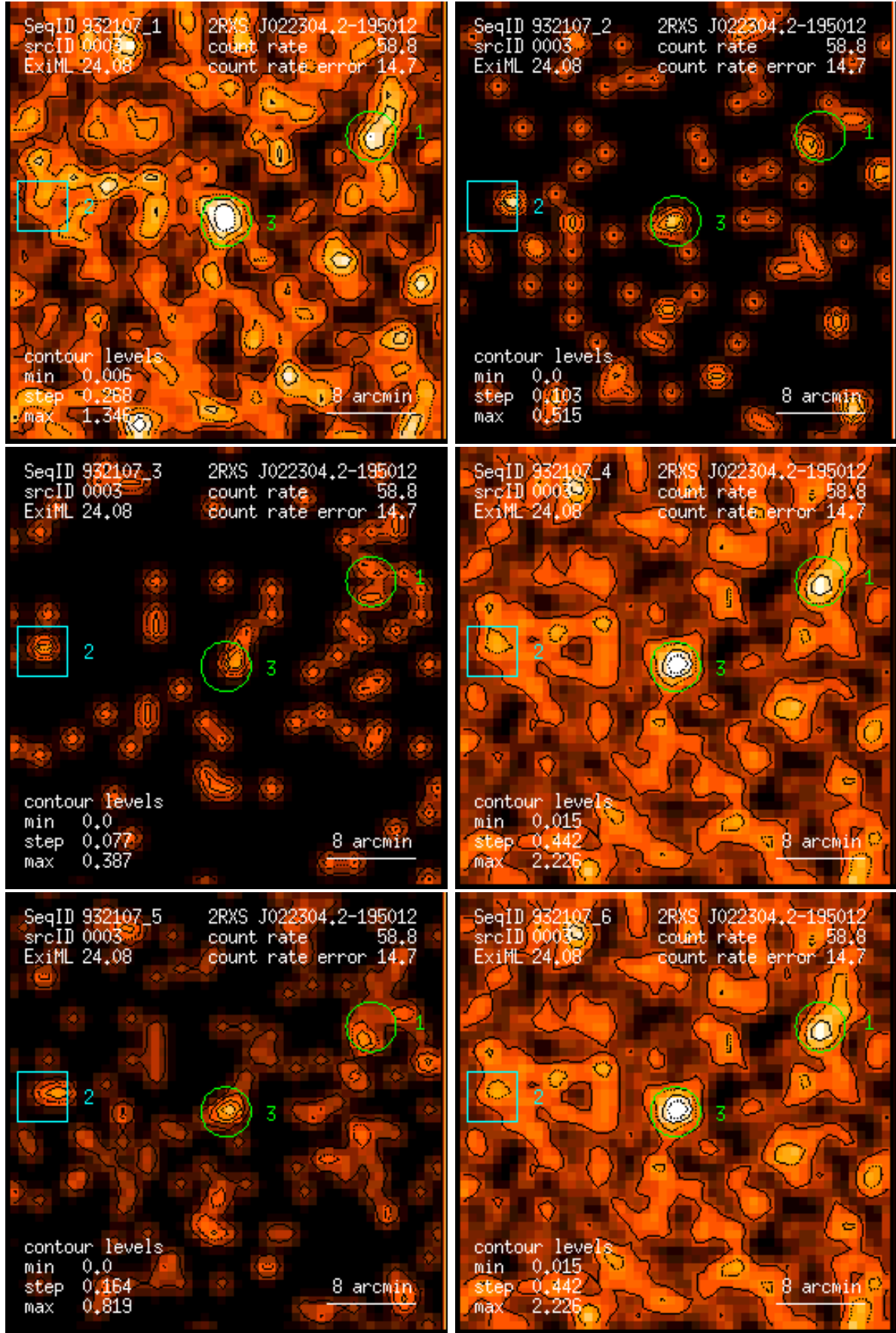
Figure 3: RASS 932107: detection 0003: band rate images, Gaussian filter: (1) PSPC channels 11 – 41, (2) 52 – 90, (3) 91 – 201, (4) 11 – 235, (5) 52 – 201, (6) 11 – 201. Broad band rates in counts/ks. Band rate contour levels in counts/ks/arcmin 2 .
