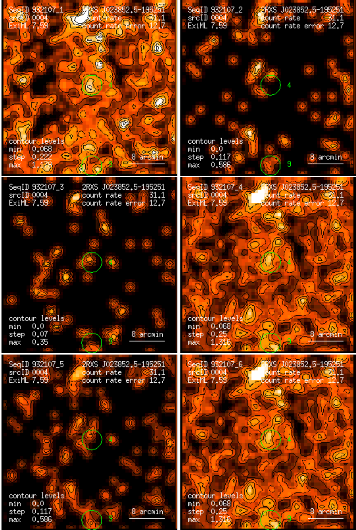
Figure 4: RASS 932107: detection 0004: band rate images, Gaussian filter: (1) PSPC channels 11 – 41, (2) 52 – 90, (3) 91 – 201, (4) 11 – 235, (5) 52 – 201, (6) 11 – 201. Broad band rates in counts/ks. Band rate contour levels in counts/ks/arcmin 2 .
