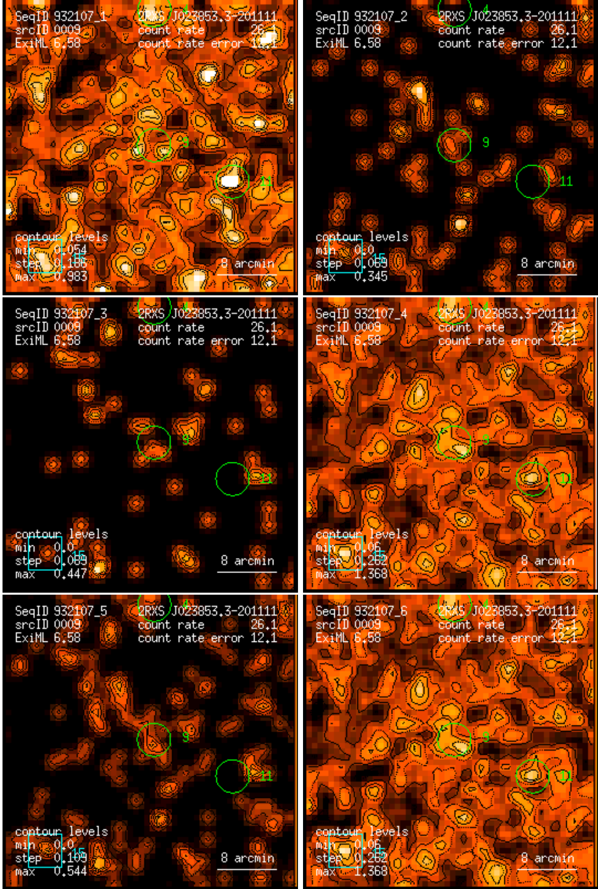
Figure 9: RASS 932107: detection 0009: band rate images, Gaussian filter: (1) PSPC channels 11 – 41, (2) 52 – 90, (3) 91 – 201, (4) 11 – 235, (5) 52 – 201, (6) 11 – 201. Broad band rates in counts/ks. Band rate contour levels in counts/ks/arcmin 2 .
