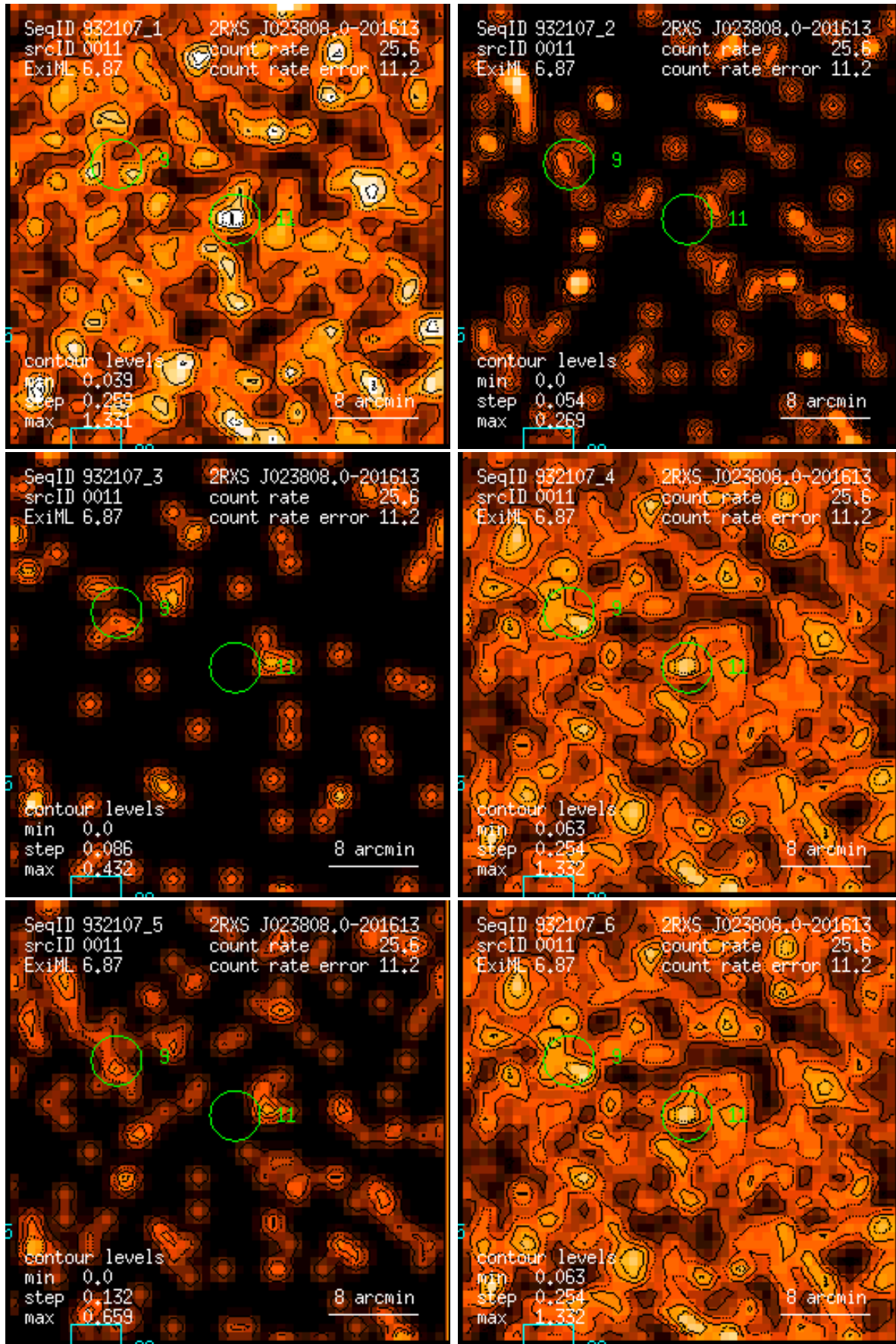
Figure 11: RASS 932107: detection 0011: band rate images, Gaussian filter: (1) PSPC channels 11 – 41, (2) 52 – 90, (3) 91 – 201, (4) 11 – 235, (5) 52 – 201, (6) 11 – 201. Broad band rates in counts/ks. Band rate contour levels in counts/ks/arcmin 2 .
