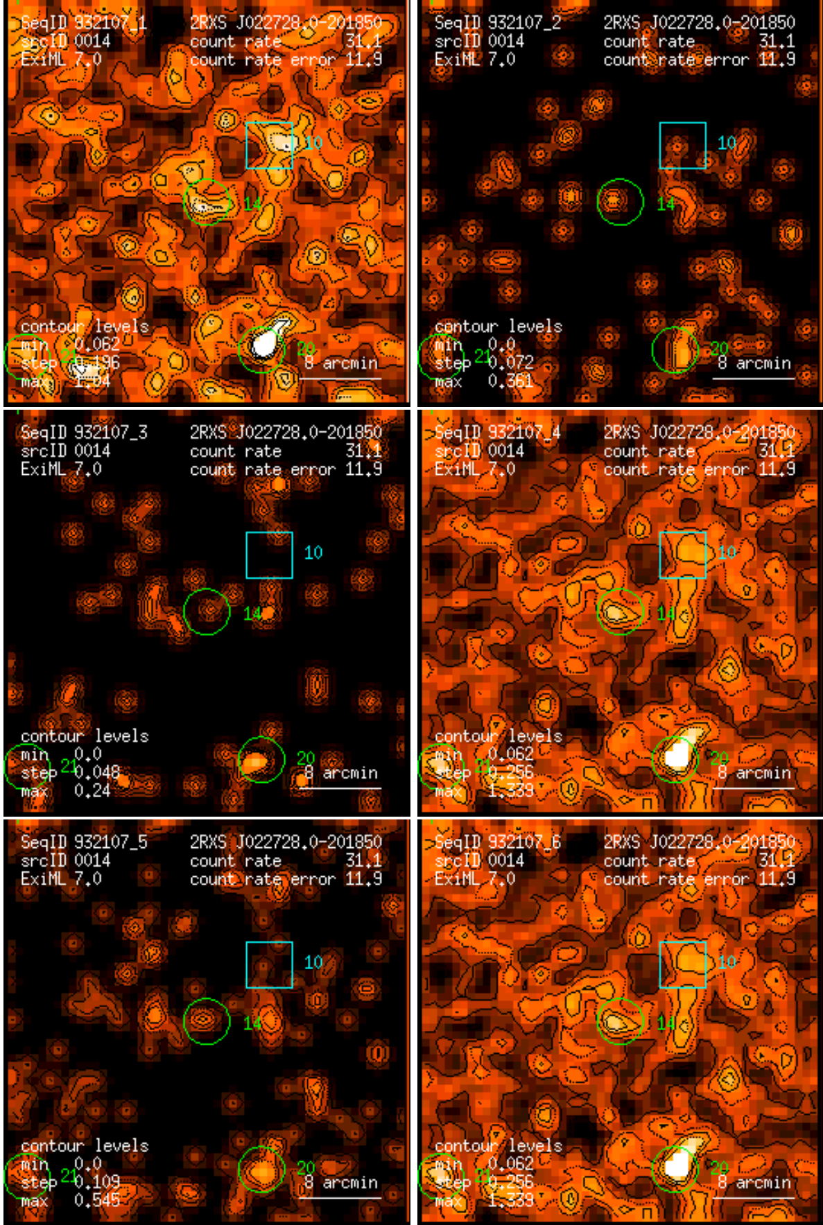
Figure 14: RASS 932107: detection 0014: band rate images, Gaussian filter: (1) PSPC channels 11 – 41, (2) 52 – 90, (3) 91 – 201, (4) 11 – 235, (5) 52 – 201, (6) 11 – 201. Broad band rates in counts/ks. Band rate contour levels in counts/ks/arcmin 2 .
