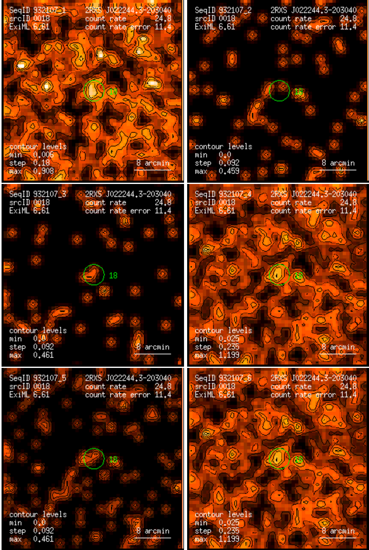
Figure 18: RASS 932107: detection 0018: band rate images, Gaussian filter: (1) PSPC channels 11 – 41, (2) 52 – 90, (3) 91 – 201, (4) 11 – 235, (5) 52 – 201, (6) 11 – 201. Broad band rates in counts/ks. Band rate contour levels in counts/ks/arcmin 2 .
