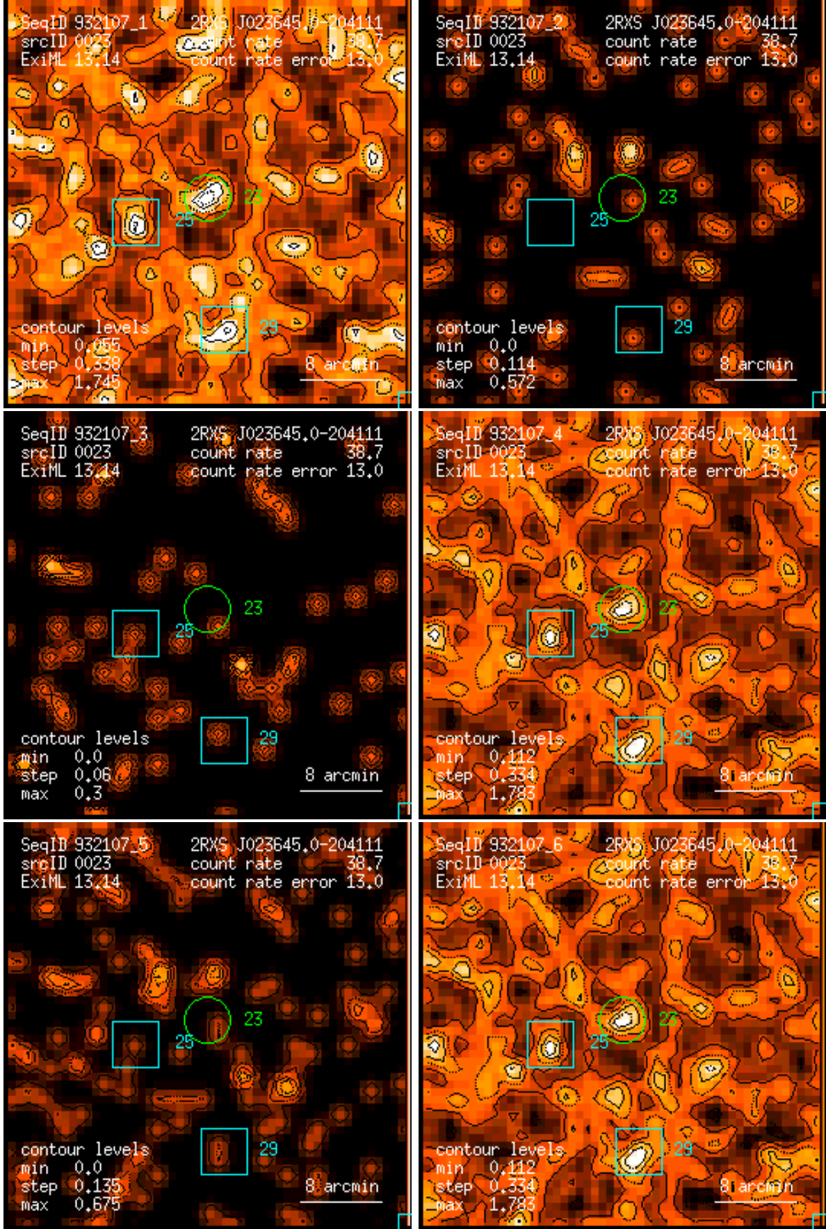
Figure 23: RASS 932107: detection 0023: band rate images, Gaussian filter: (1) PSPC channels 11 – 41, (2) 52 – 90, (3) 91 – 201, (4) 11 – 235, (5) 52 – 201, (6) 11 – 201. Broad band rates in counts/ks. Band rate contour levels in counts/ks/arcmin 2 .
