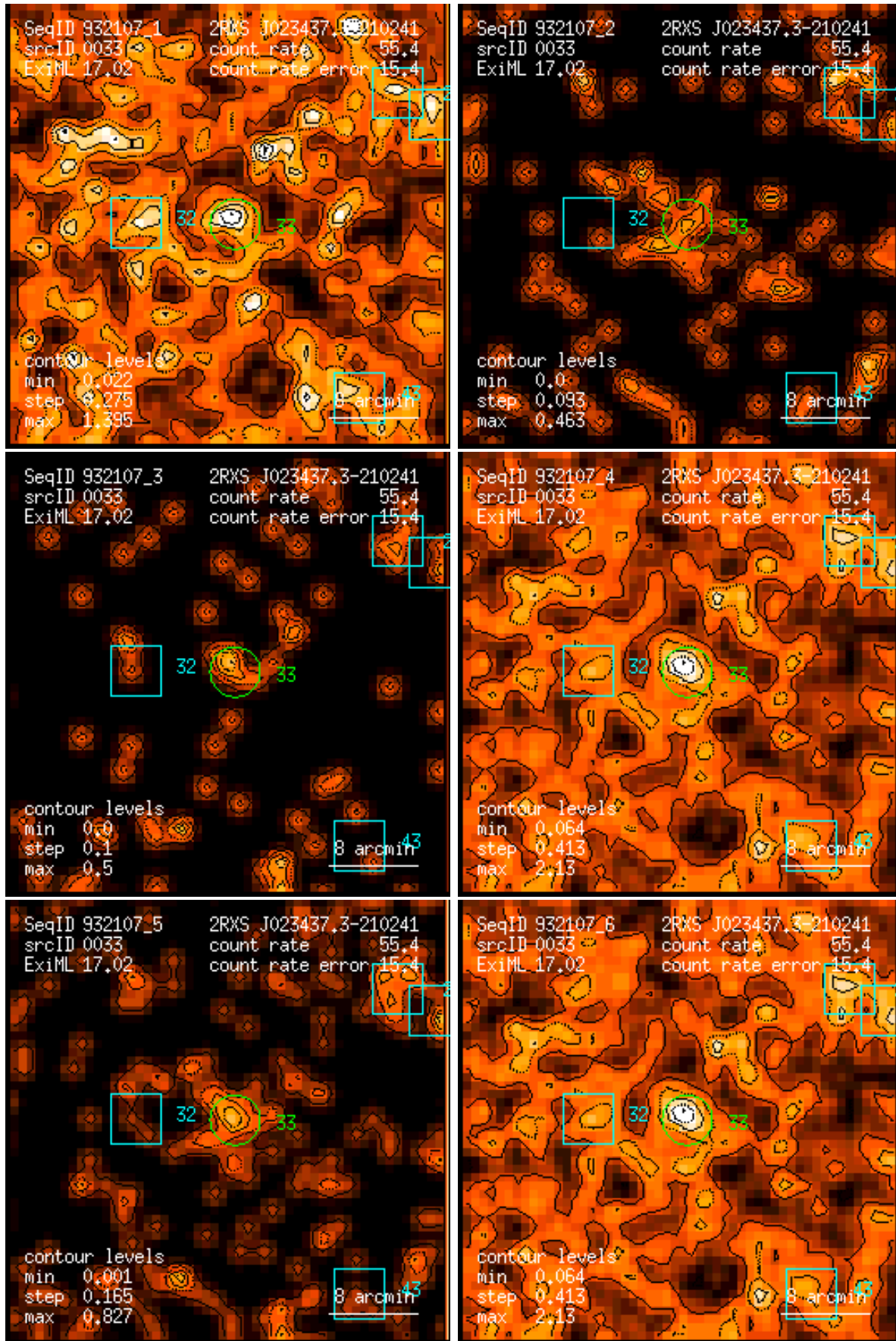
Figure 33: RASS 932107: detection 0033: band rate images, Gaussian filter: (1) PSPC channels 11 – 41, (2) 52 – 90, (3) 91 – 201, (4) 11 – 235, (5) 52 – 201, (6) 11 – 201. Broad band rates in counts/ks. Band rate contour levels in counts/ks/arcmin 2 .
