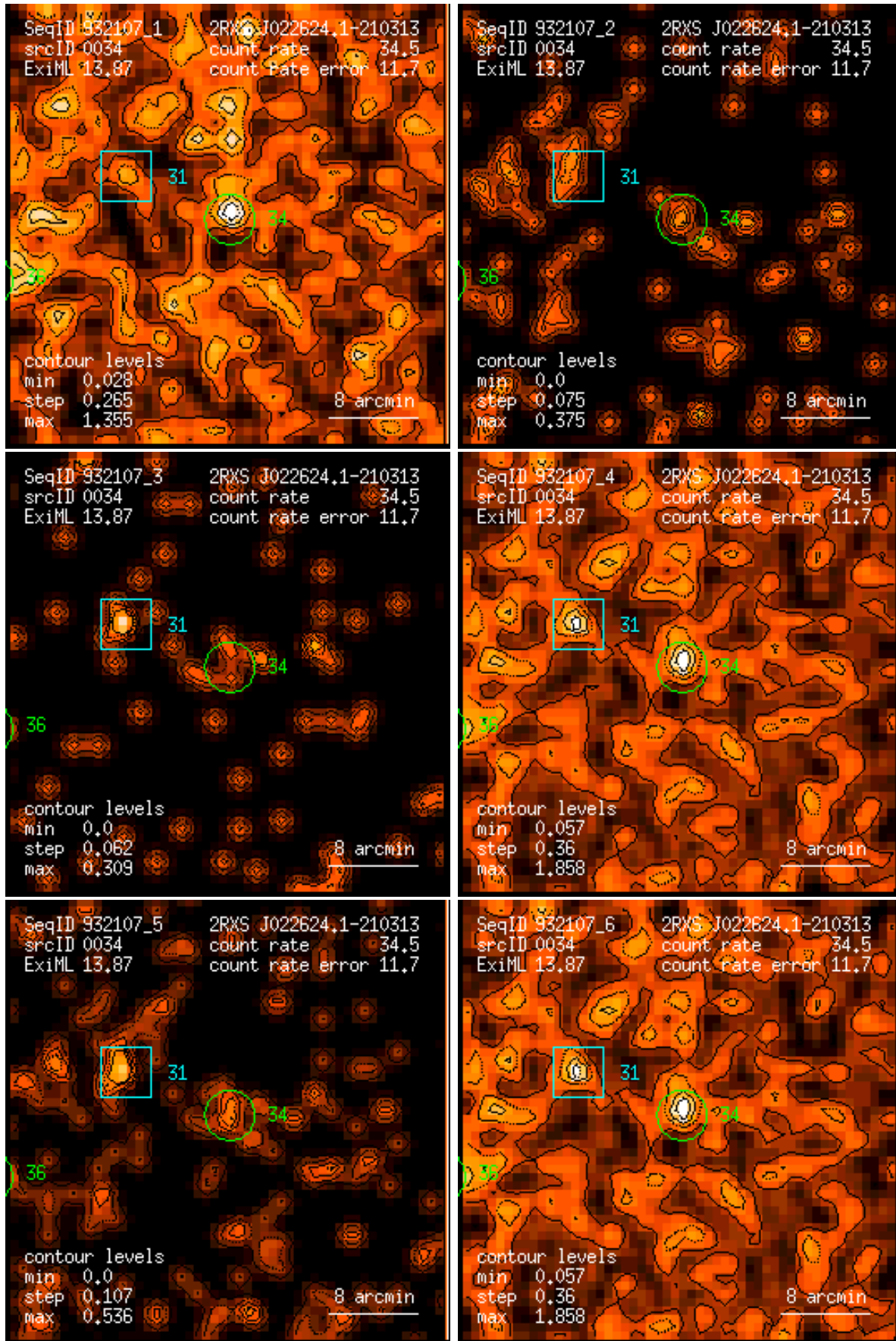
Figure 34: RASS 932107: detection 0034: band rate images, Gaussian filter: (1) PSPC channels 11 – 41, (2) 52 – 90, (3) 91 – 201, (4) 11 – 235, (5) 52 – 201, (6) 11 – 201. Broad band rates in counts/ks. Band rate contour levels in counts/ks/arcmin 2 .
