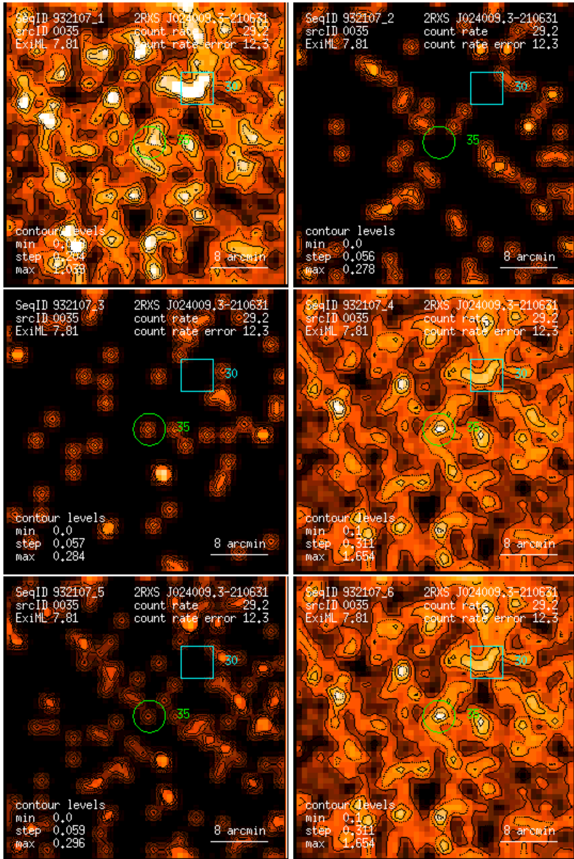
Figure 35: RASS 932107: detection 0035: band rate images, Gaussian filter: (1) PSPC channels 11 – 41, (2) 52 – 90, (3) 91 – 201, (4) 11 – 235, (5) 52 – 201, (6) 11 – 201. Broad band rates in counts/ks. Band rate contour levels in counts/ks/arcmin 2 .
