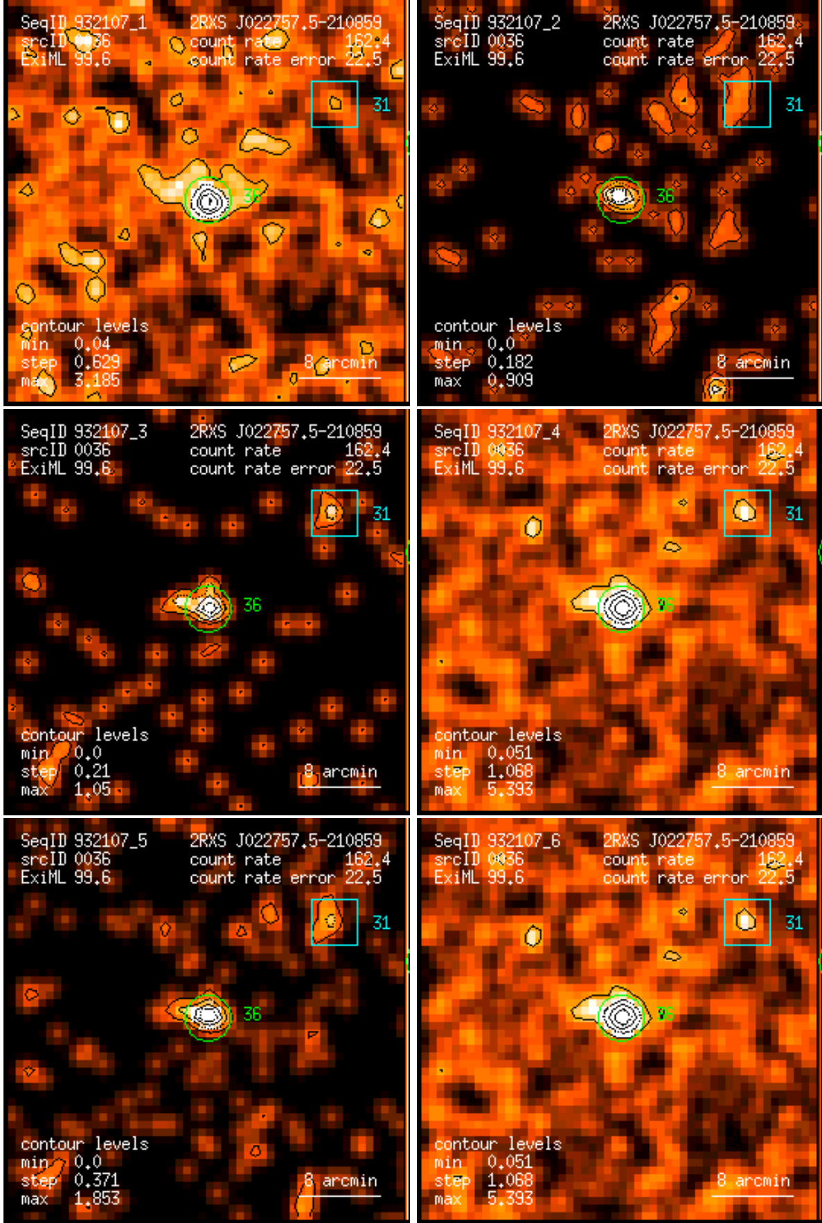
Figure 36: RASS 932107: detection 0036: band rate images, Gaussian filter: (1) PSPC channels 11 – 41, (2) 52 – 90, (3) 91 – 201, (4) 11 – 235, (5) 52 – 201, (6) 11 – 201. Broad band rates in counts/ks. Band rate contour levels in counts/ks/arcmin 2 .
