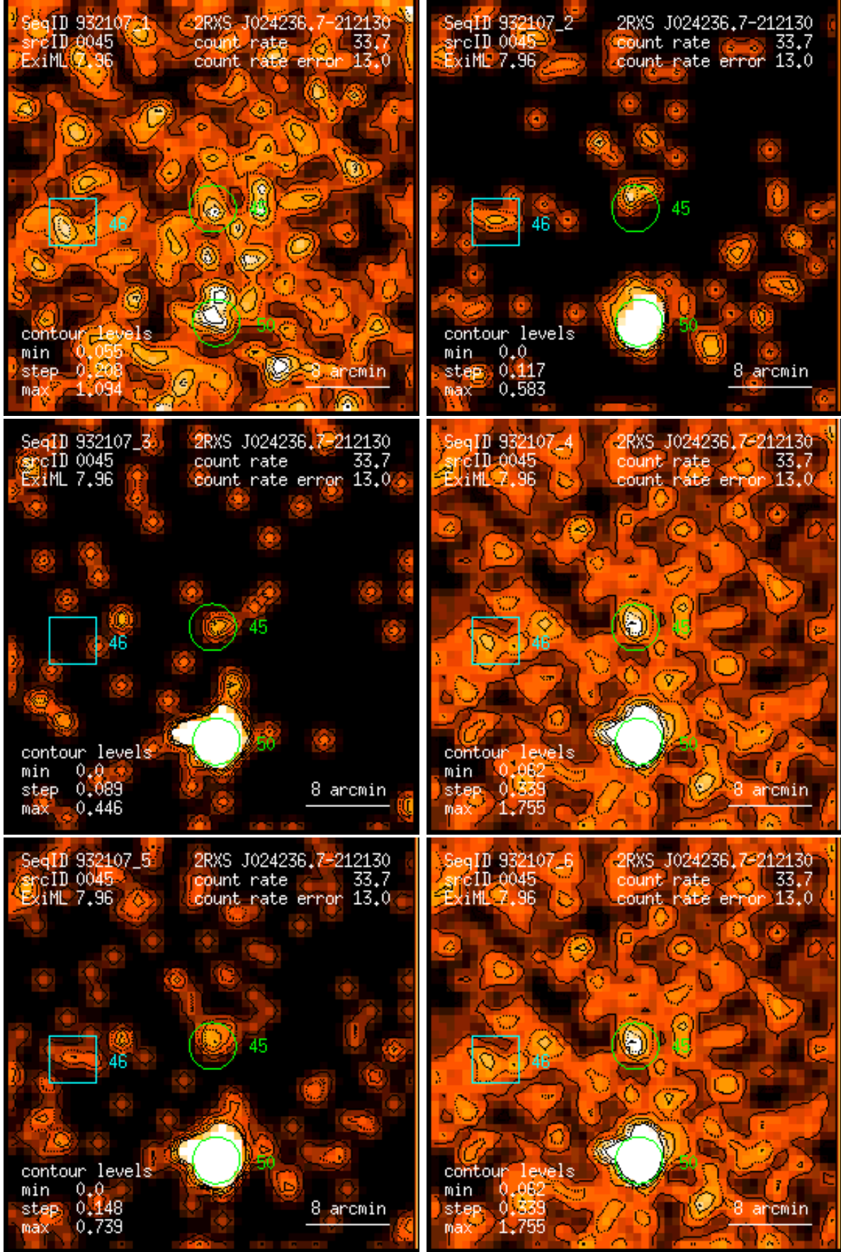
Figure 45: RASS 932107: detection 0045: band rate images, Gaussian filter: (1) PSPC channels 11 – 41, (2) 52 – 90, (3) 91 – 201, (4) 11 – 235, (5) 52 – 201, (6) 11 – 201. Broad band rates in counts/ks. Band rate contour levels in counts/ks/arcmin 2 .
