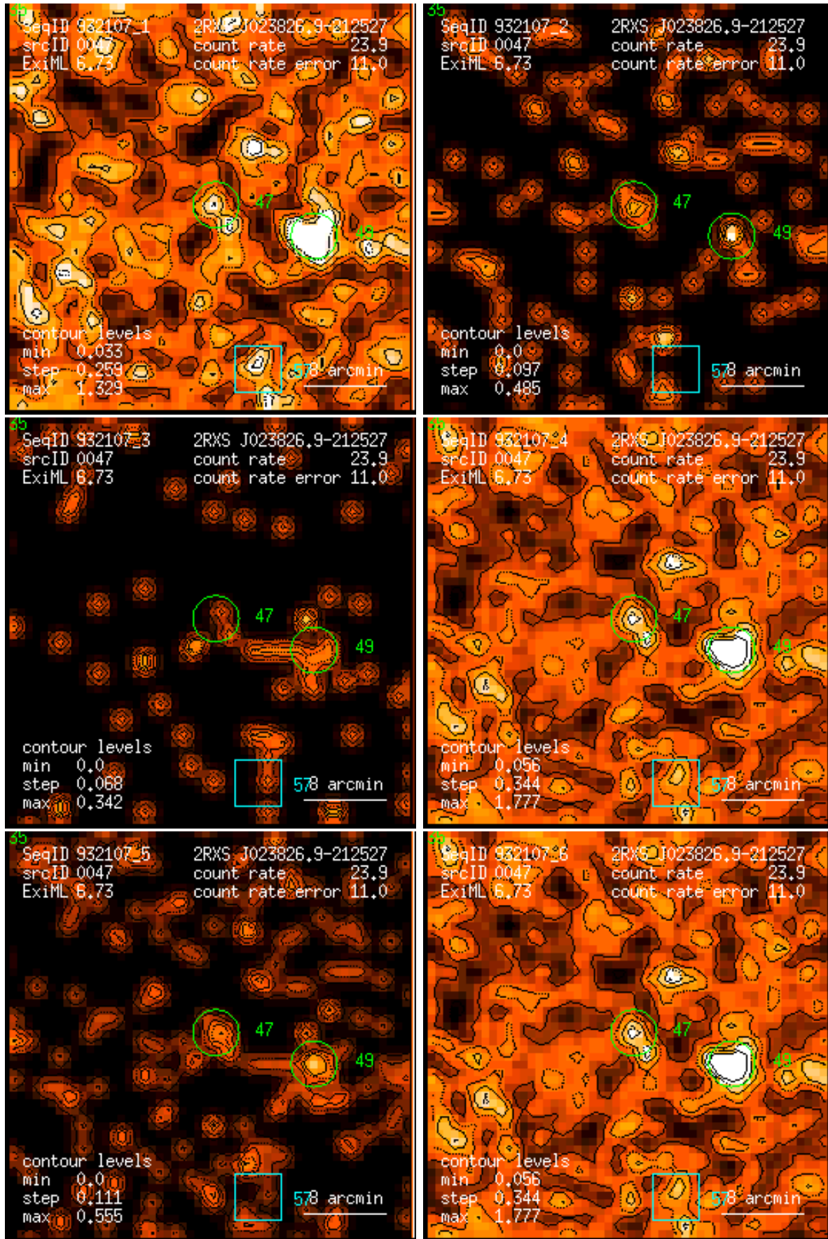
Figure 47: RASS 932107: detection 0047: band rate images, Gaussian filter: (1) PSPC channels 11 – 41, (2) 52 – 90, (3) 91 – 201, (4) 11 – 235, (5) 52 – 201, (6) 11 – 201. Broad band rates in counts/ks. Band rate contour levels in counts/ks/arcmin 2 .
